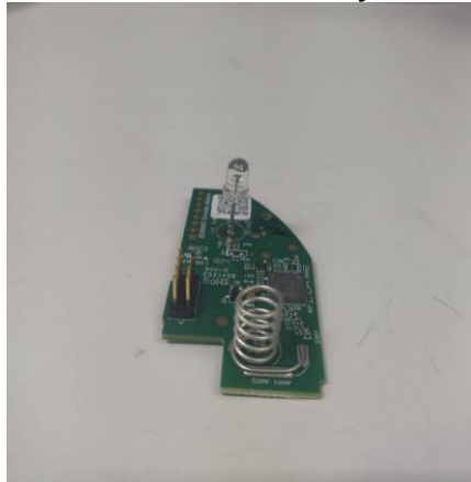
Photograph No.4 Smoke and heat detector Antenna assembly
