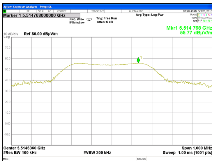
Plot 7.7.34 Radiated emission measurements at the seventh harmonic of low carrier frequency
