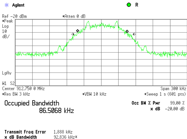
Plot 7.1.4 The 99% occupied bandwidth at low frequency
