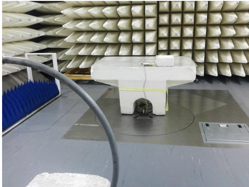
Photograph No.3 Setup for spurious field strength measurements in anechoic chamber from 9 kHz to 30 MHz
