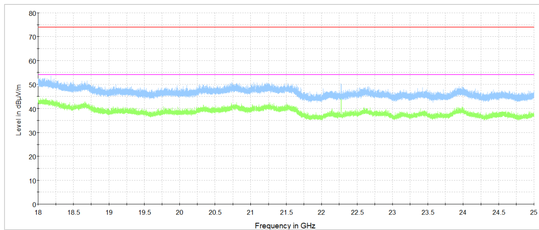
Plot 7.3.50 Radiated emission measurements from 18000 to 25000 MHz at the high carrier frequency 2480 MHz Antenna 2
