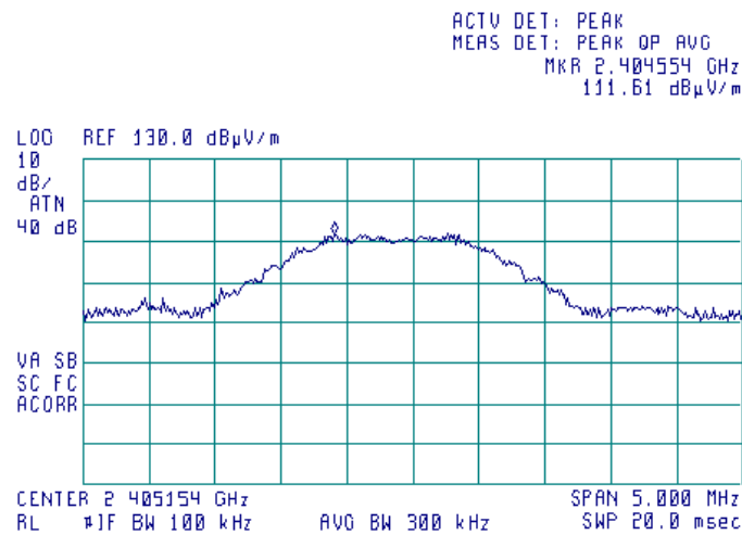
Plot 7.4.2 The highest emission level within the assigned band at low carrier frequency ch.11, Antenna 2
