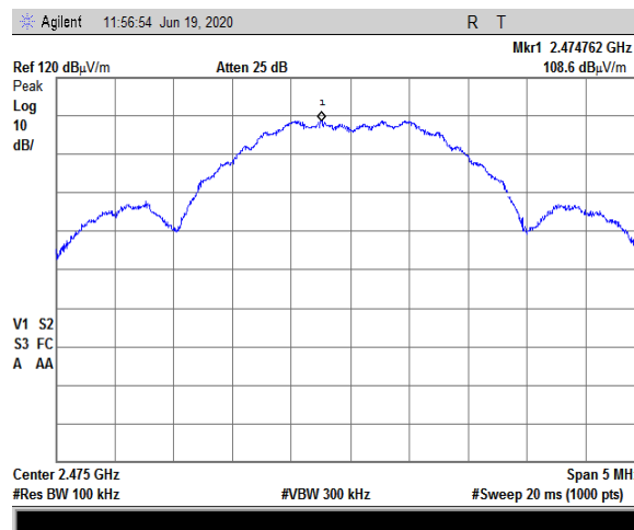
Plot 7.3.8 Radiated emission measurements at the high carrier frequency Ch.26, Antenna 2
