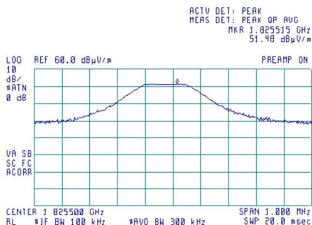
Plot 7.7.23 Radiated emission measurements at the second harmonic of mid carrier frequency
