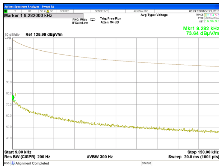
Plot 7.7.8 Radiated emission measurements from 9 to 150 kHz at the mid carrier frequency
