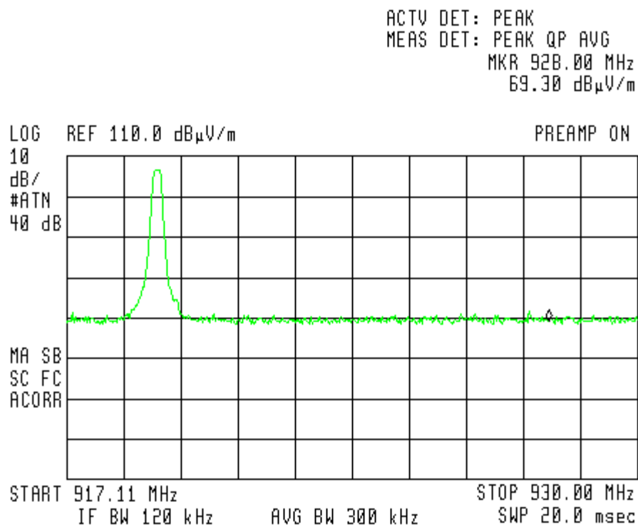
Figure 49 — 928.0 MHz Horizontal – Ceiling Mounted – Continuous Mode
