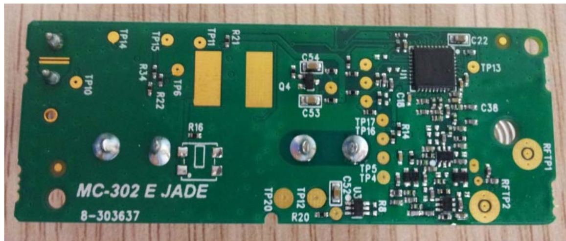
Photograph No.2 Flood detector PCB rear side view
