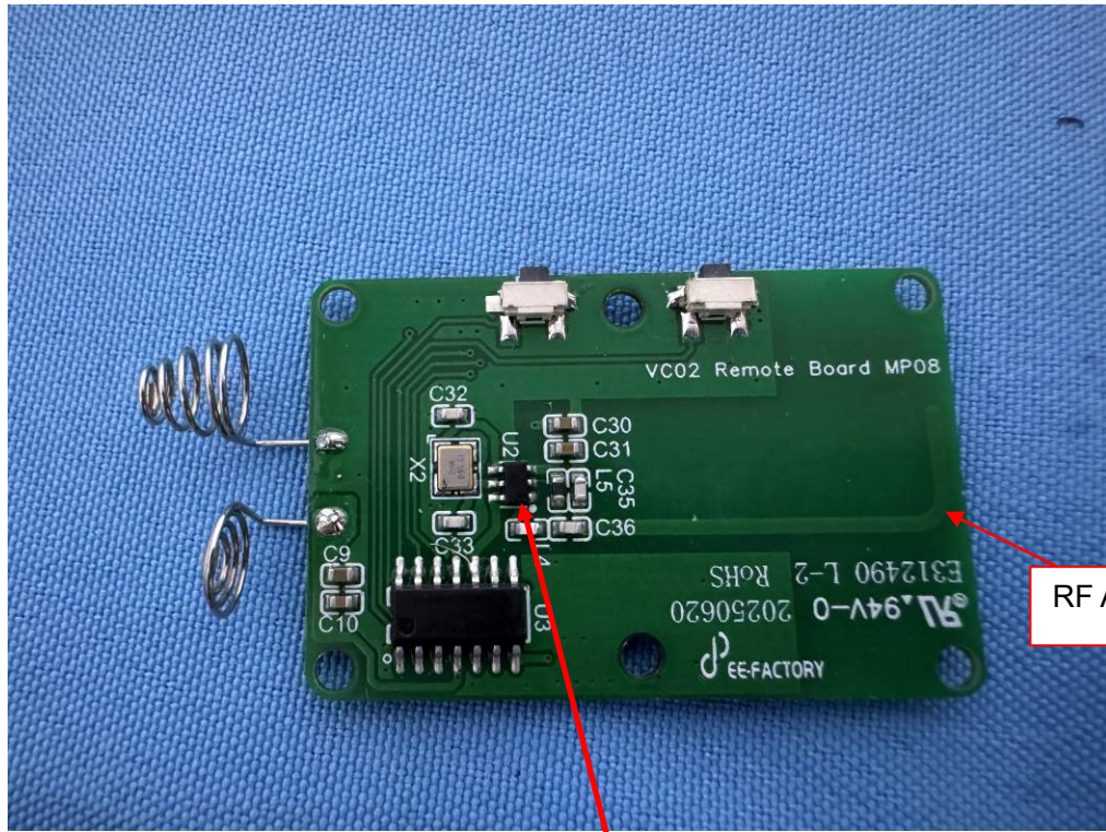
RF Chip
