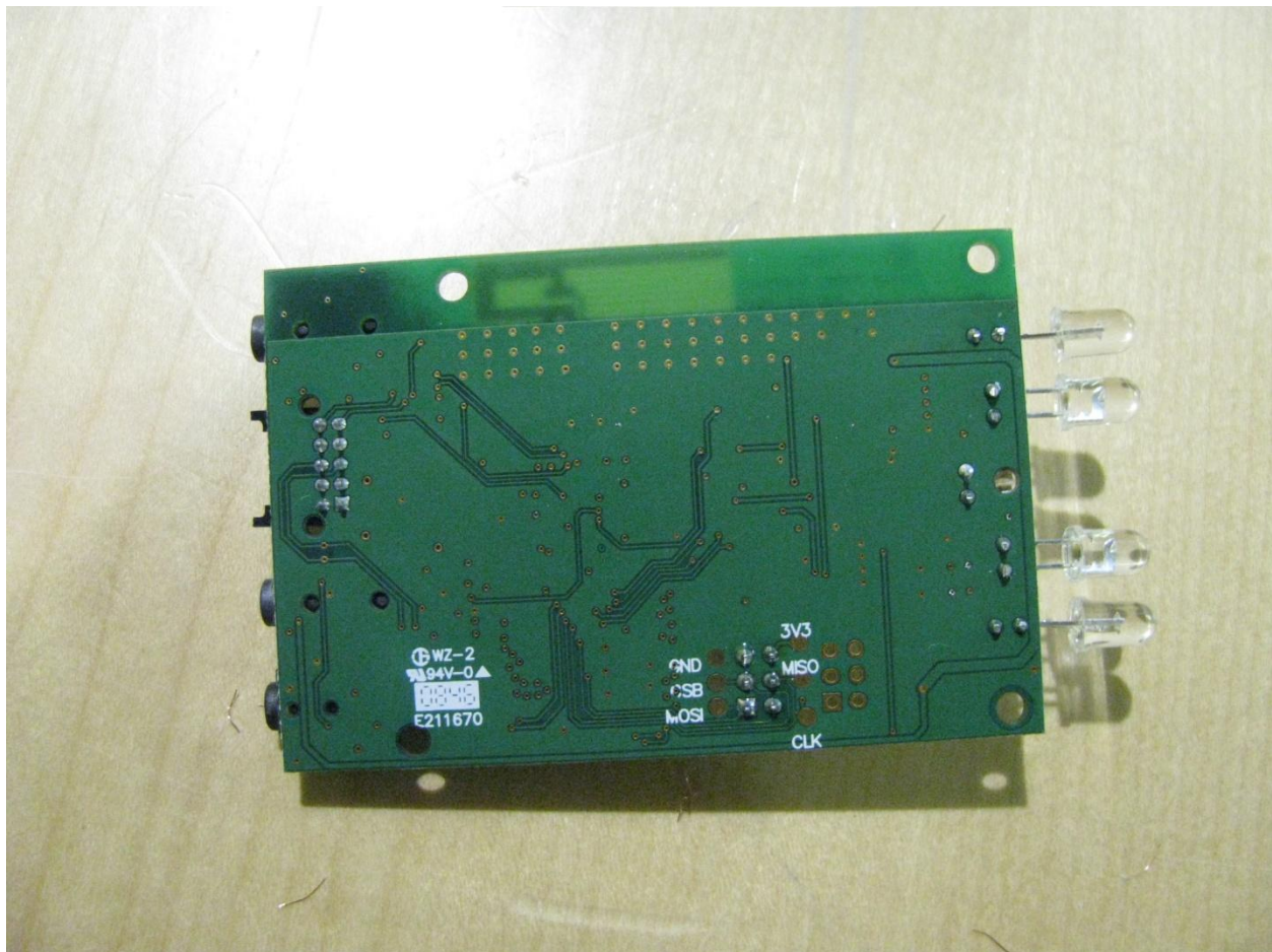
Figure 2 – Bottom side of board
