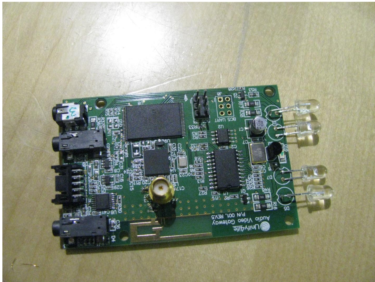
Figure 3 – SMA connector provided for conducted measurements (for testing only)
