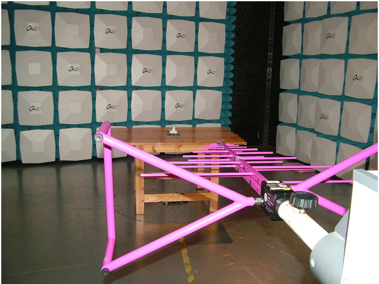
Photograph 1: Radiated Emissions
