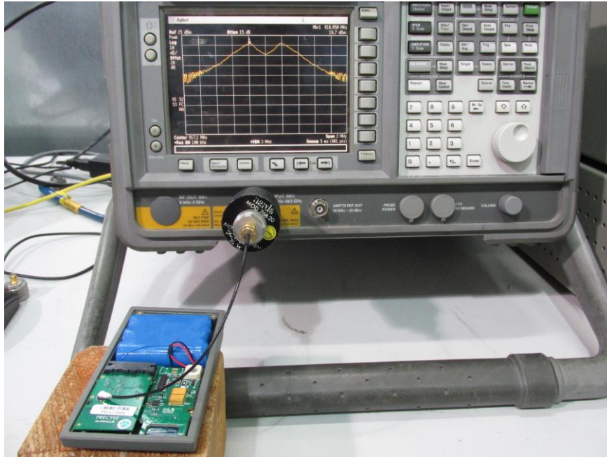
Photograph 3: Conducted Measurements
