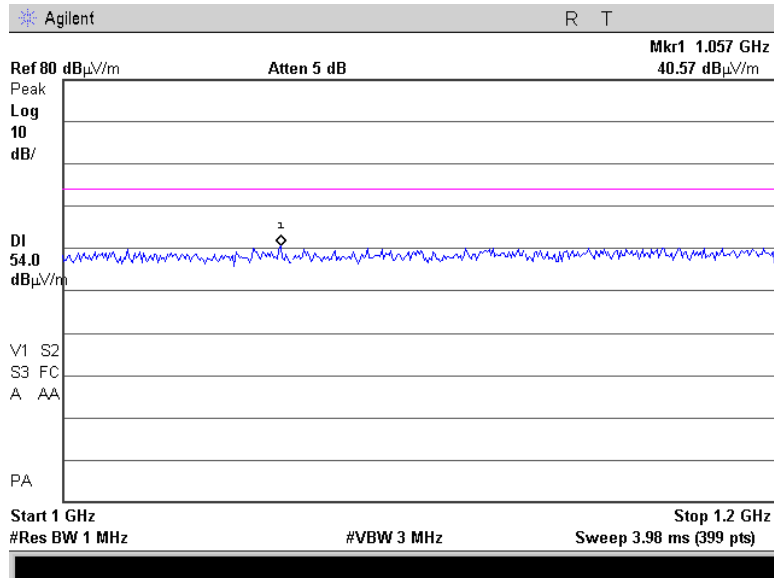
Plot 4.5.5 Unwanted Radiated Emissions in 1 – 1.2 GHz range, Fc = 917.14 MHz Horizontal & Vertical Polarization
