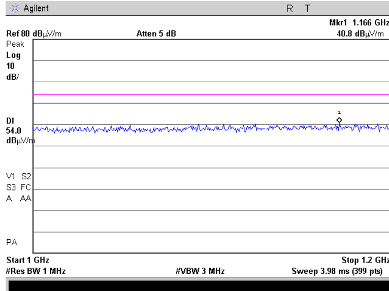
Plot 4.5.10 Unwanted Radiated Emissions in 1 – 1.2 GHz range, Fc = 911.47 MHz Horizontal & Vertical Polarization
