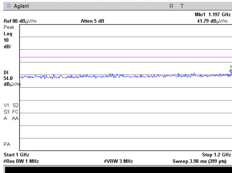
Plot 4.5.12 Unwanted Radiated Emissions in 1 – 1.2 GHz range, Fc = 917.14 MHz Horizontal & Vertical Polarization
