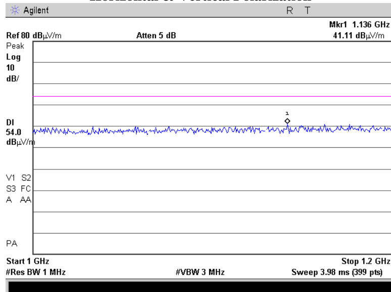
Plot 4.5.3 Unwanted Radiated Emissions in 1 – 1.2 GHz range, Fc = 911.47 MHz Horizontal & Vertical Polarization
