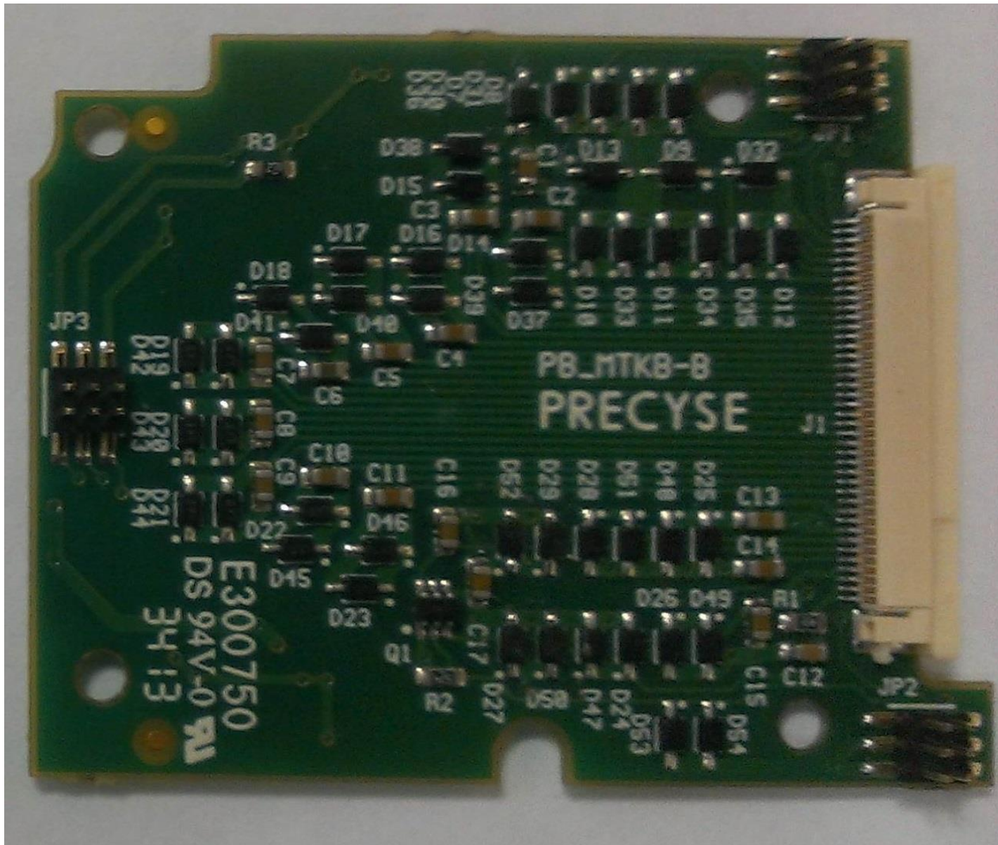
Photograph 1: PB_MTKB-B Front screen not attached
