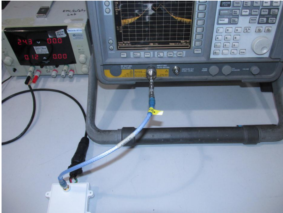
Photograph 1: Conducted Power Measurements
