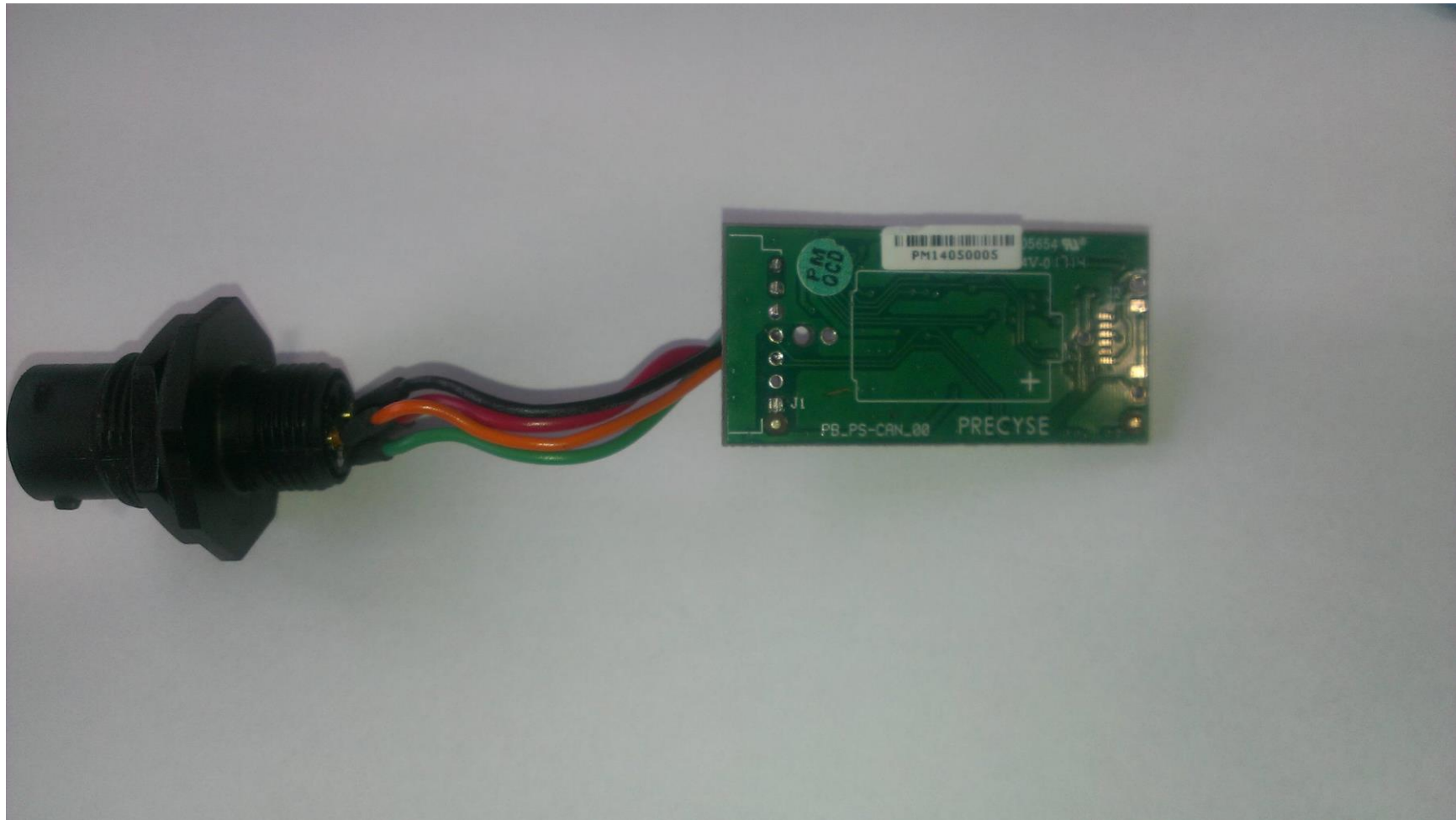
Figure 7 - PS-CAN Bottom
