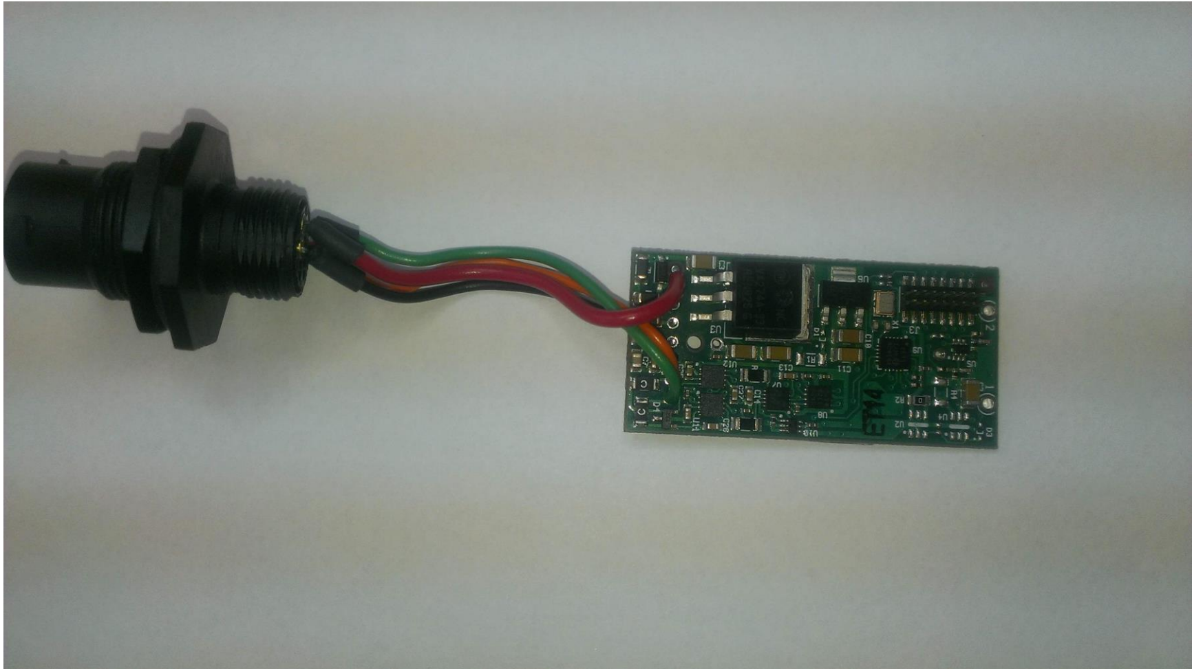
Figure 5 – PS-CAN Top
