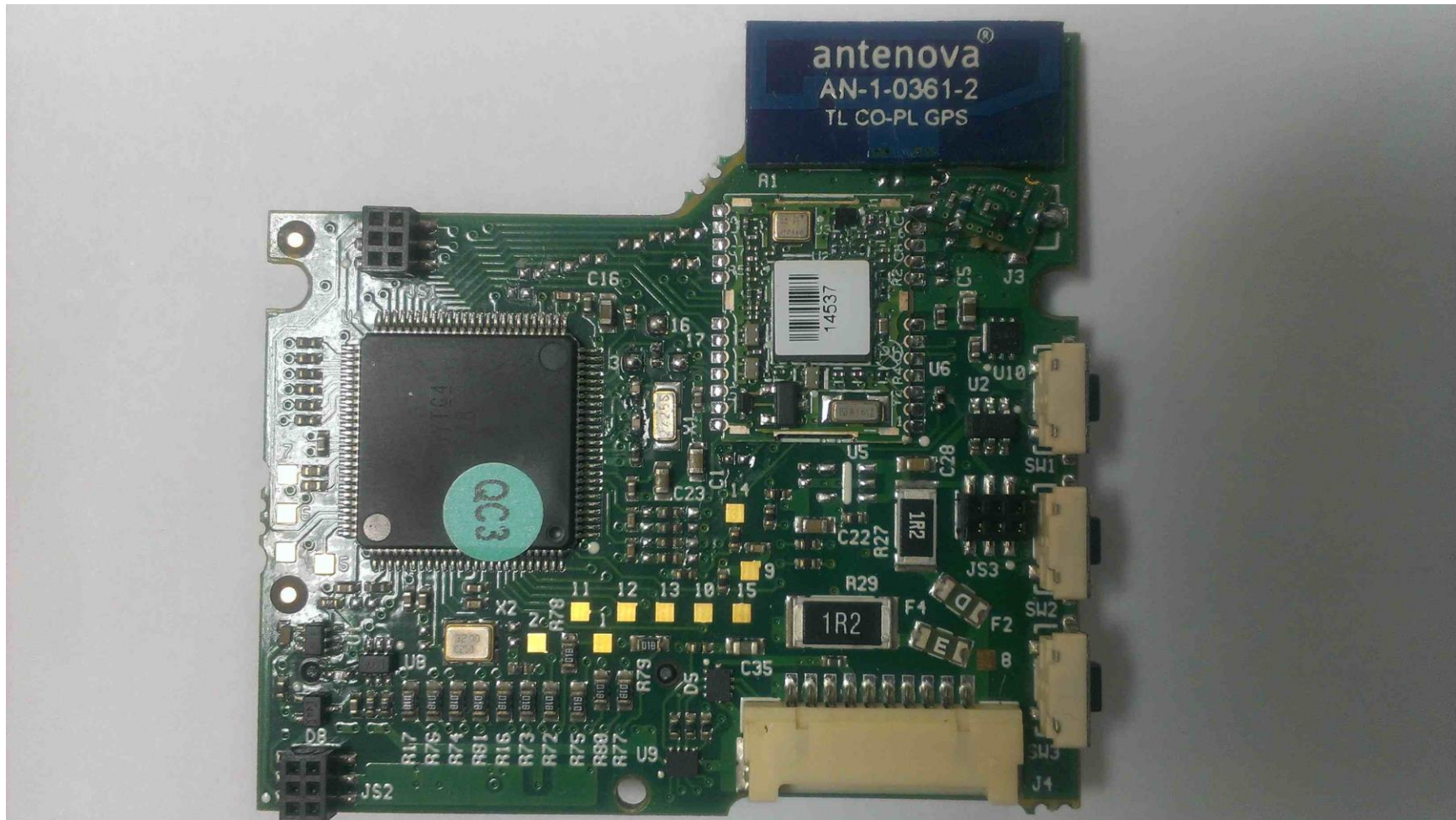
Figure 3 -MTMB-B.B1 Top
