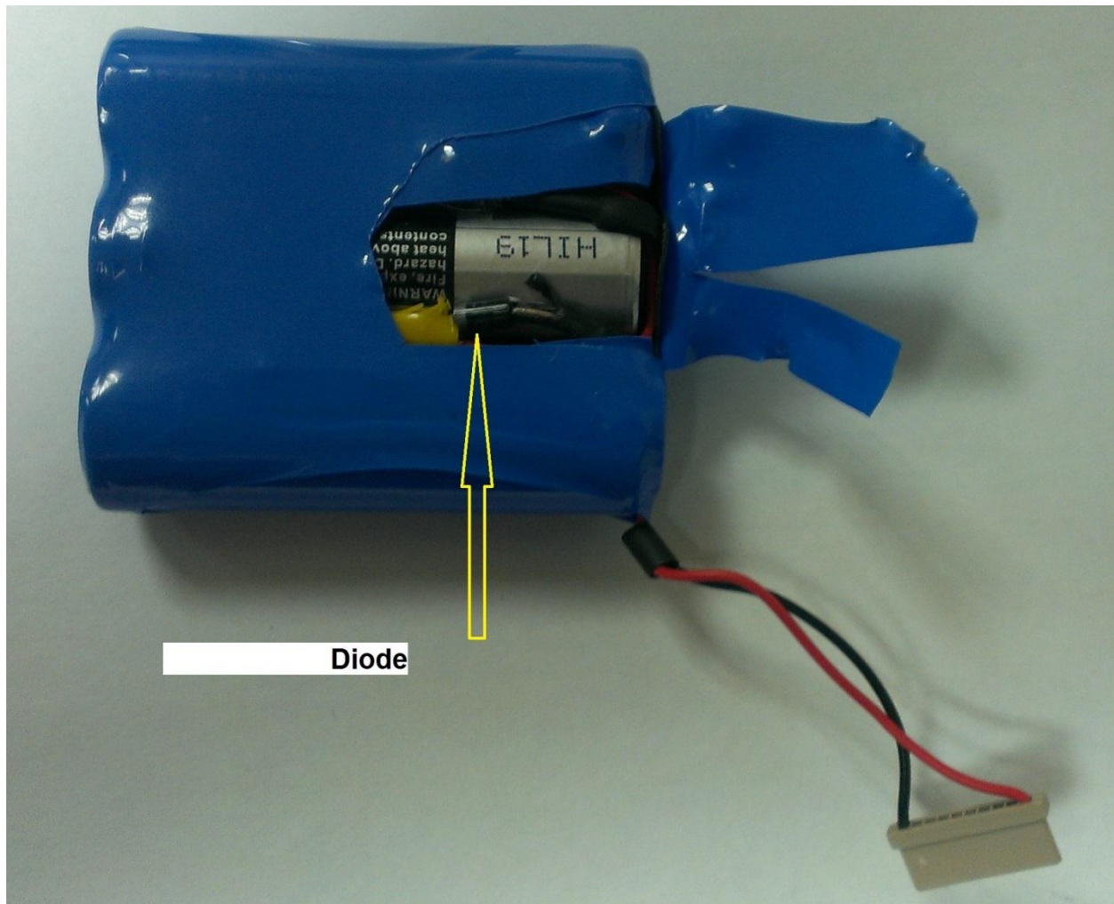
B. Picture of the inside of the battery pack.
