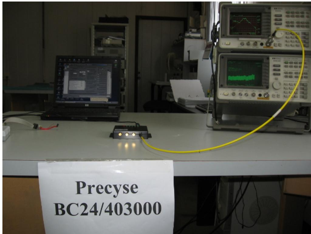
Conducted Emission From Antenna Ports Tests Set-up
