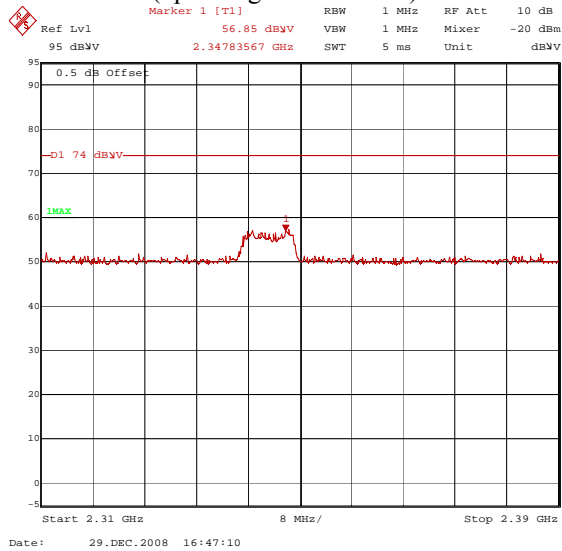
Figure 7. Plot of the Band Edge (Radiated)
