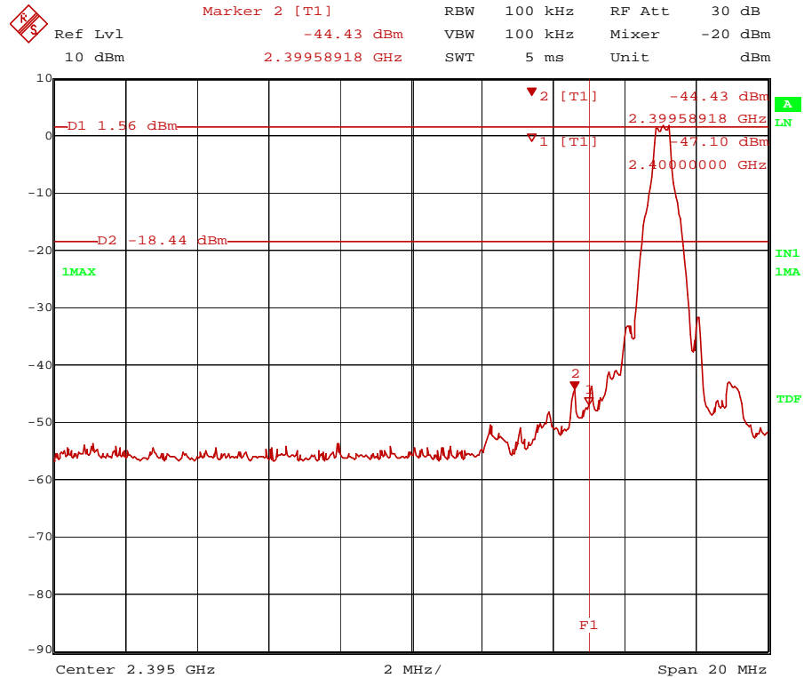
Figure 6. Plot of the Band Edge (Conducted)
