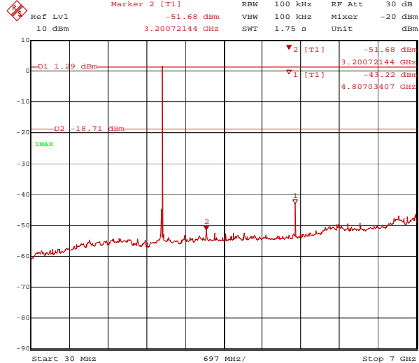
Figure 8: Spurious RF conducted emissions
