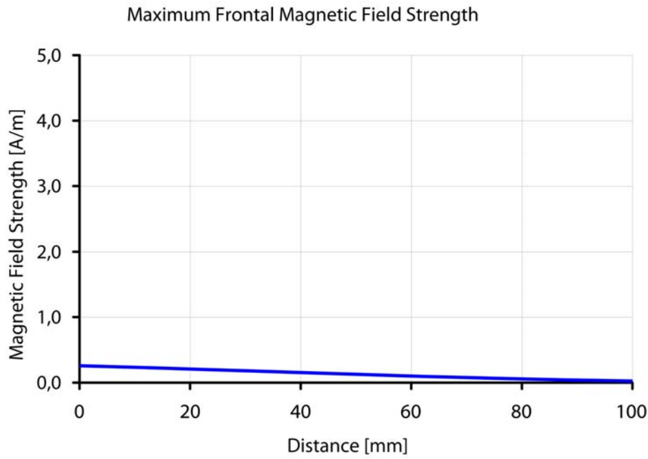
Figure 4.4 Magnetic field strength frontal
