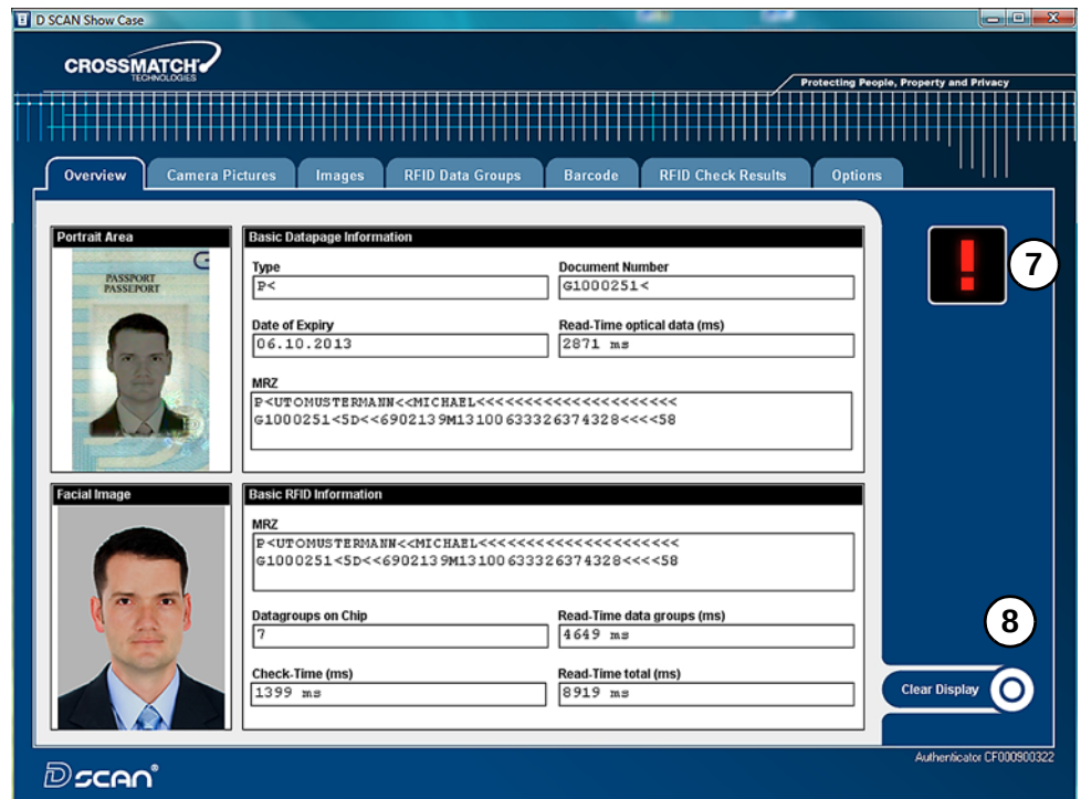
Figure 3.8 Failed verification
