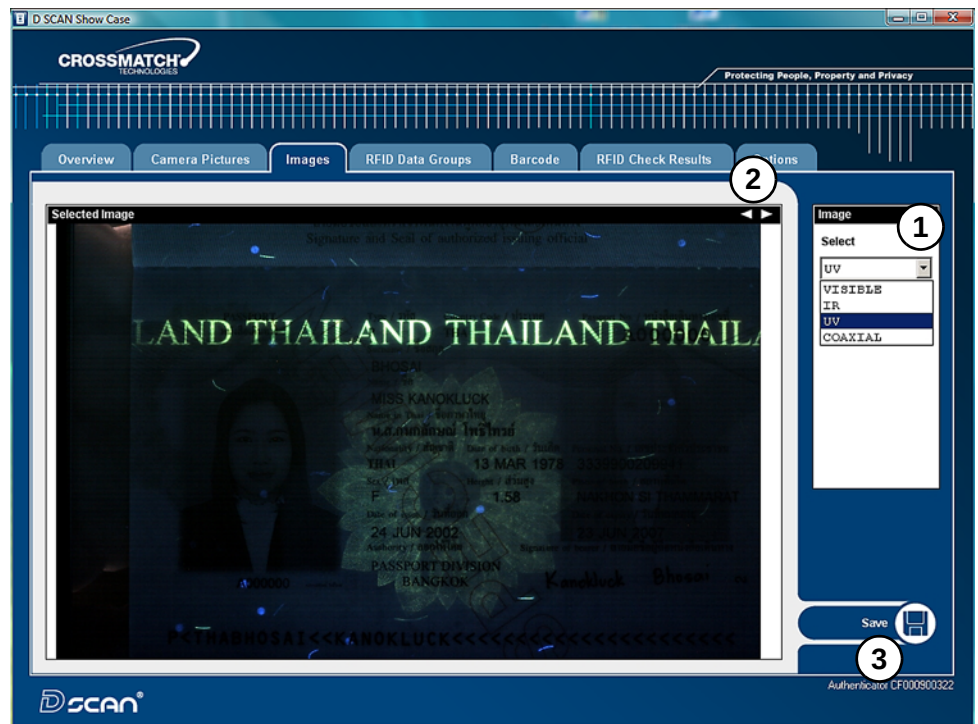
Figure 3.10 Images page
