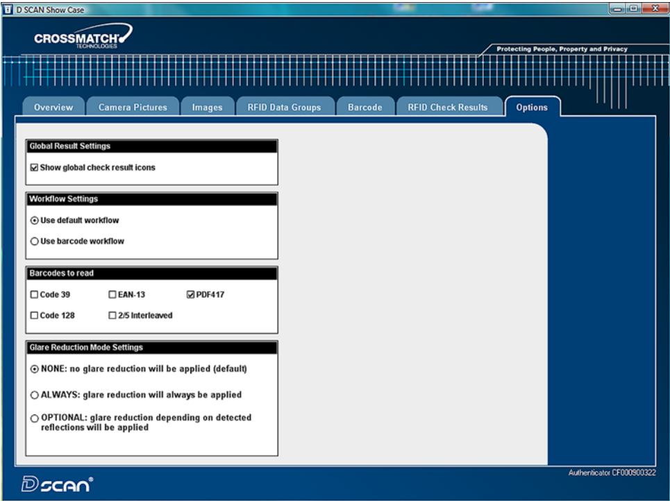
Figure 3.14 Options page
