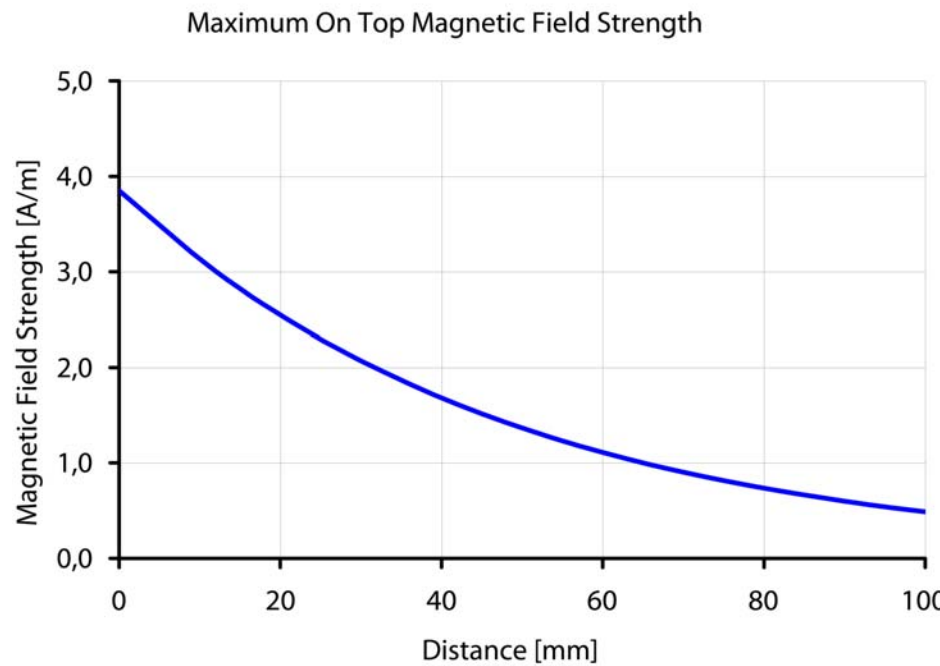
Figure 4.5 Magnetic field strength on top
