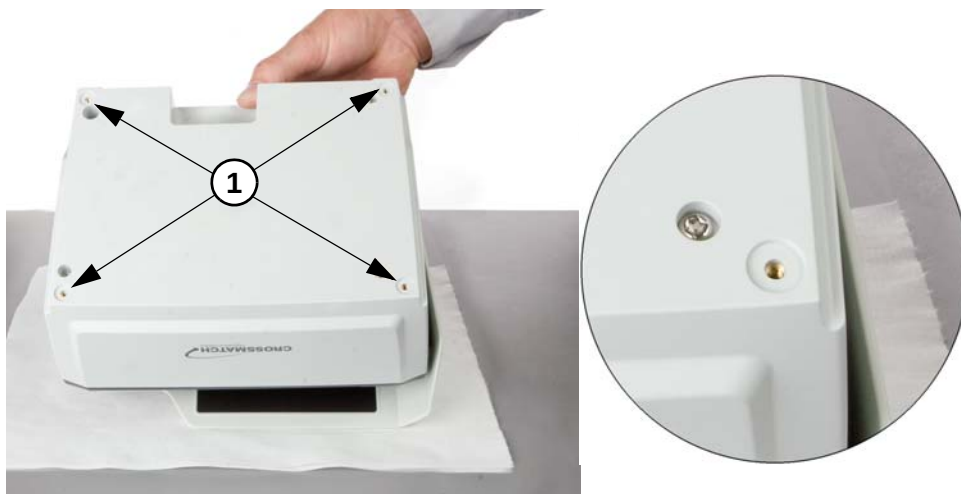
Figure 2.10 Mount points
