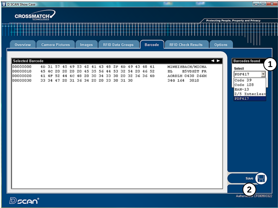
Figure 3.12 Barcode page
