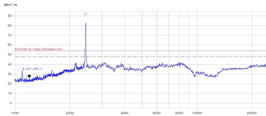
(Plot B.5: Antenna Vertical, 1GHz to 25GHz)
