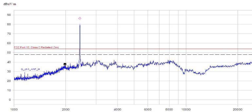
(Plot A.3: Antenna Horizontal, 1GHz to 25GHz)
