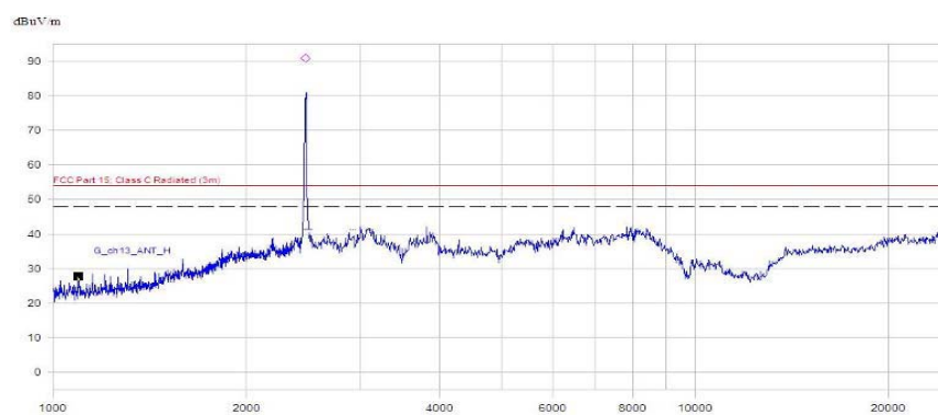
(Plot C.3: Antenna Horizontal, 1GHz to 25GHz)
