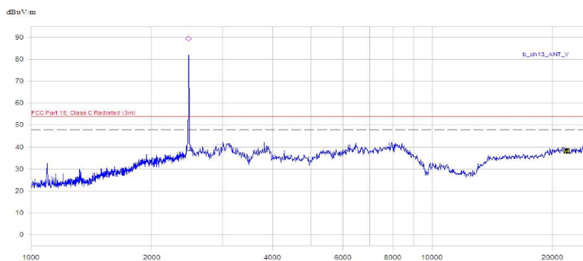
(Plot C.7: Antenna Vertical, 1GHz to 25GHz)
