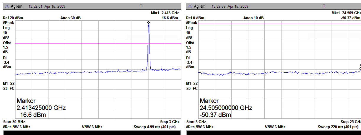
(Plot D.1: Channel = 1, 30MHz to 25GHz)
