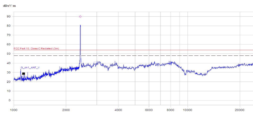
(Plot A.5: Antenna Vertical, 1GHz to 25GHz)
