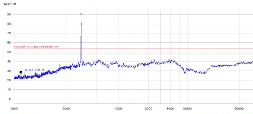
(Plot B.3: Antenna Horizontal, 1GHz to 25GHz)
