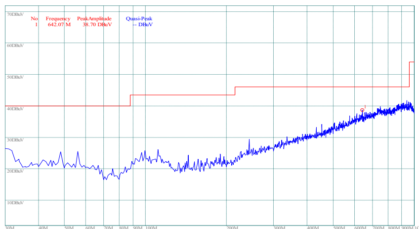
(Plot C.2: Antenna Horizontal, 30MHz to 1GHz)
