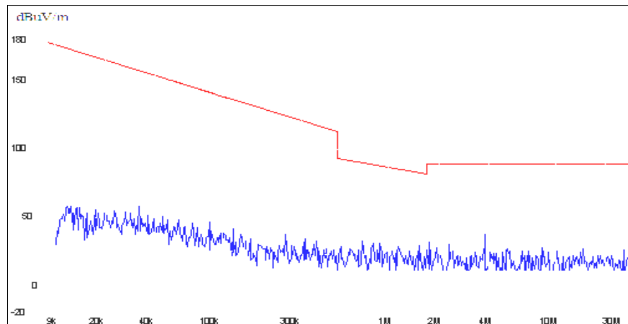
(Plot C.1: 9kHz to 30MHz)
