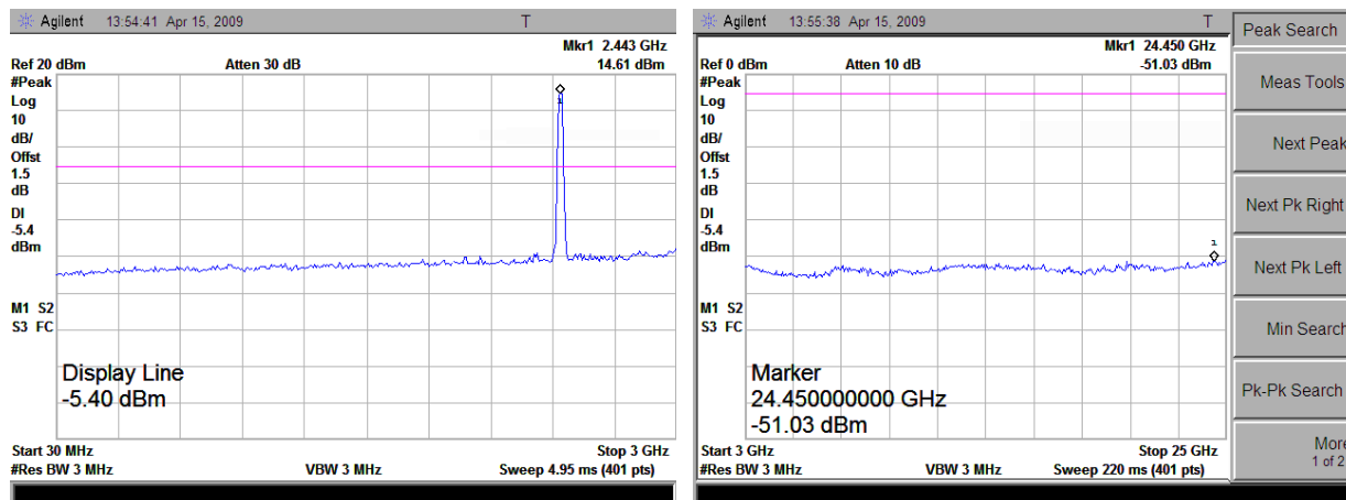
(Plot E.1: Channel = 7, 30MHz to 25GHz)
