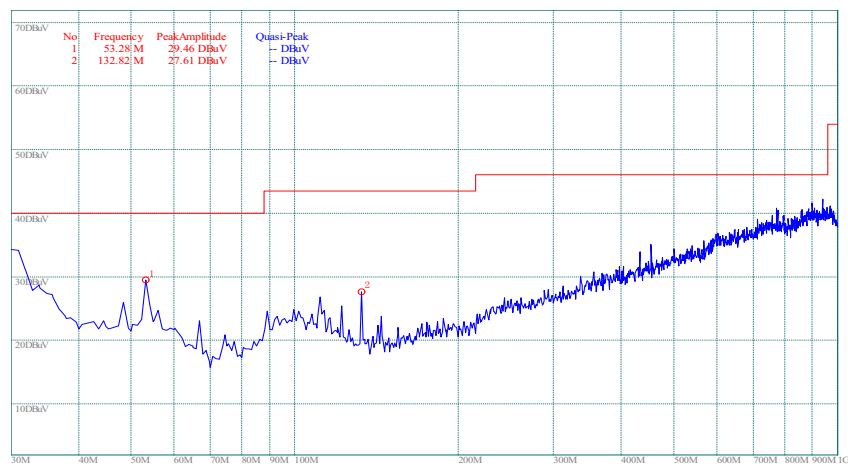
(Plot C.6: Antenna Vertical, 30MHz to 1GHz)
