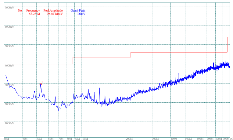
(Plot C.6: Antenna Vertical, 30MHz to 1GHz)
