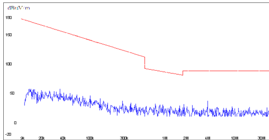
(Plot A.1: 9kHz to 30MHz)
