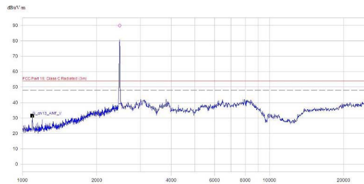
(Plot C.7: Antenna Vertical, 1GHz to 25GHz)
