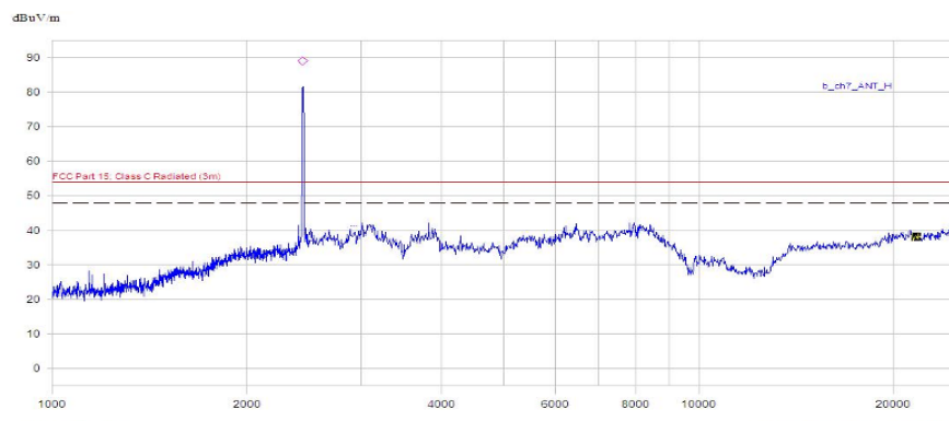
(Plot B.3: Antenna Horizontal, 1GHz to 25GHz)
