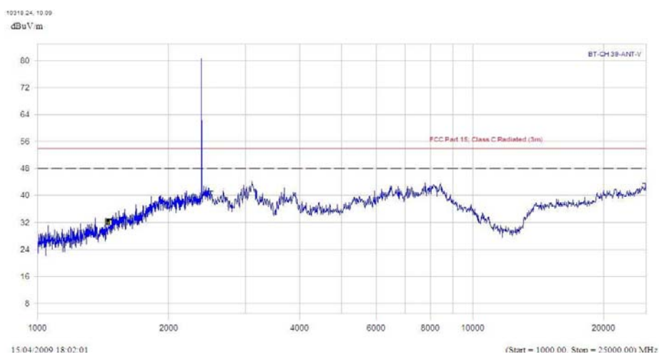
(Plot B.6: Antenna Vertical, 1GHz to 25GHz)
