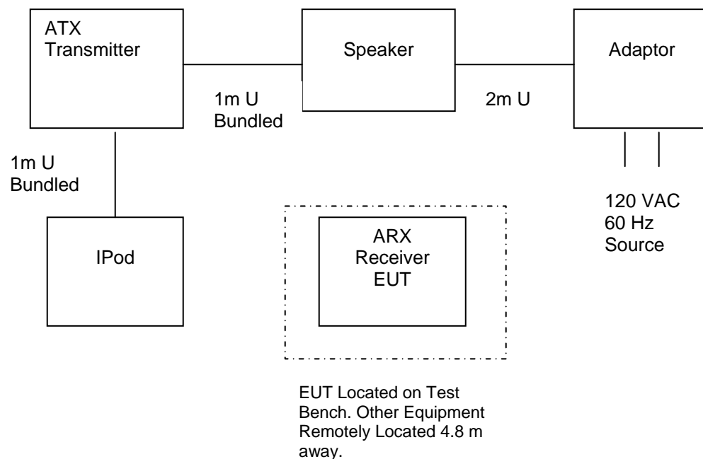
Figure 3. Test Configuration
