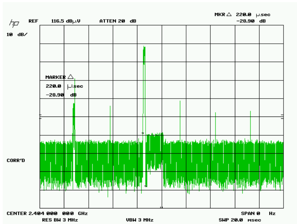
Figure 1(a). ARX Transmitter Pulse Width (Longer Pulses).
