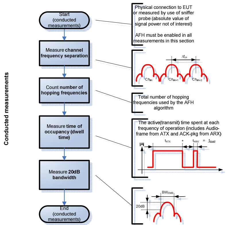
Figure 2.b – Compliance test measurement flowchart (conducted)
