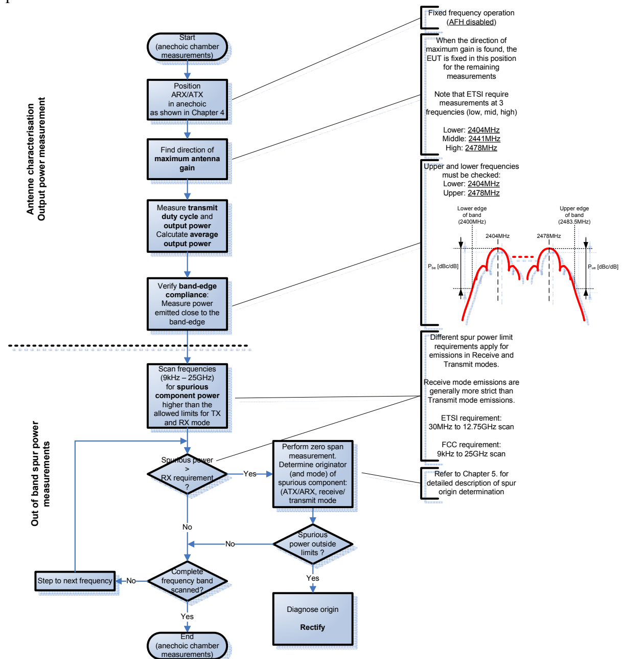
Figure 2.a – Compliance test measurement flowchart (radiated)
