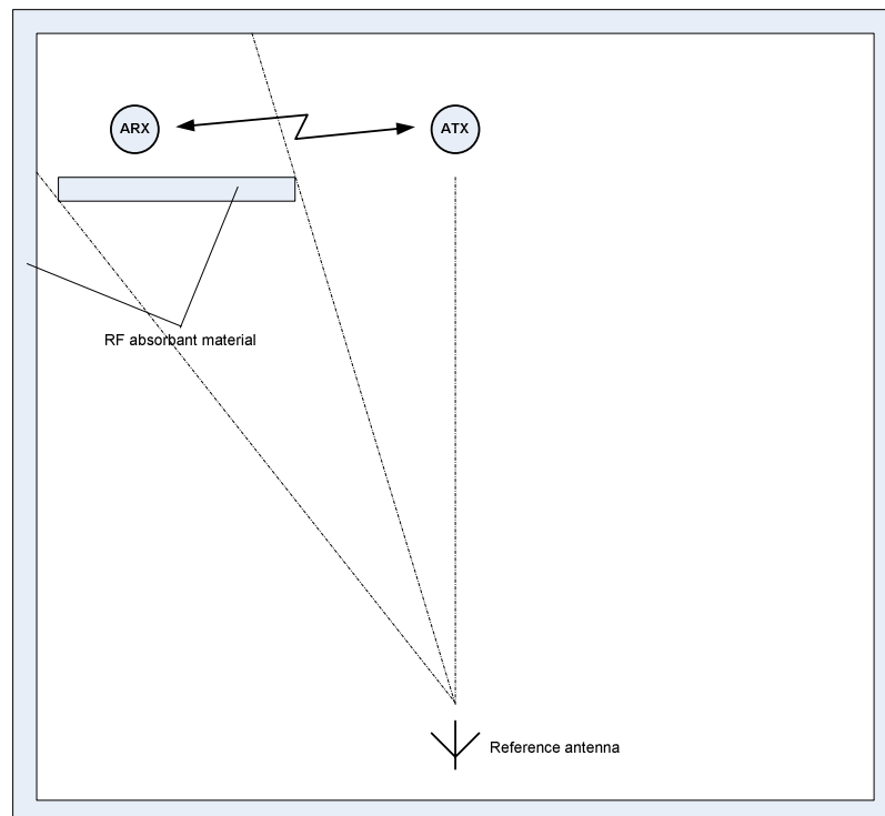
Figure 7 – Anechoic chamber measurement principle.
