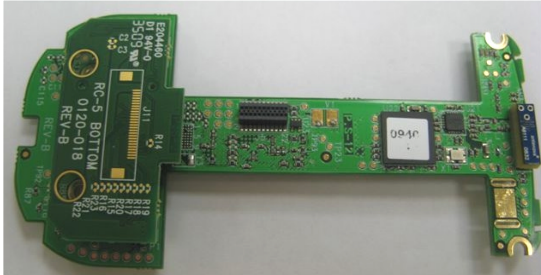
Photograph No.6 Remote Control middle PCB bottom view
