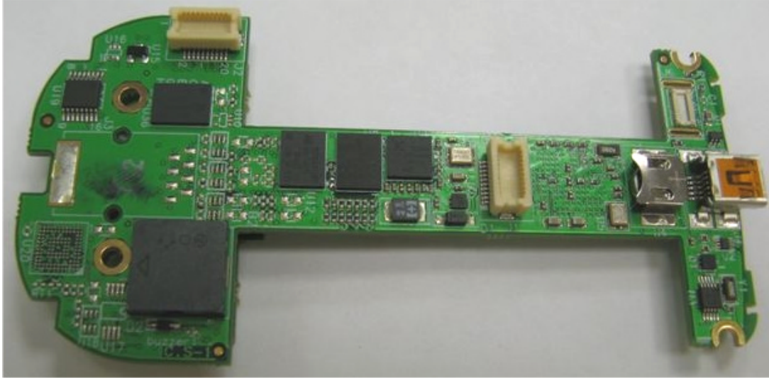
Photograph No.8 Remote Control middle PCB top view
