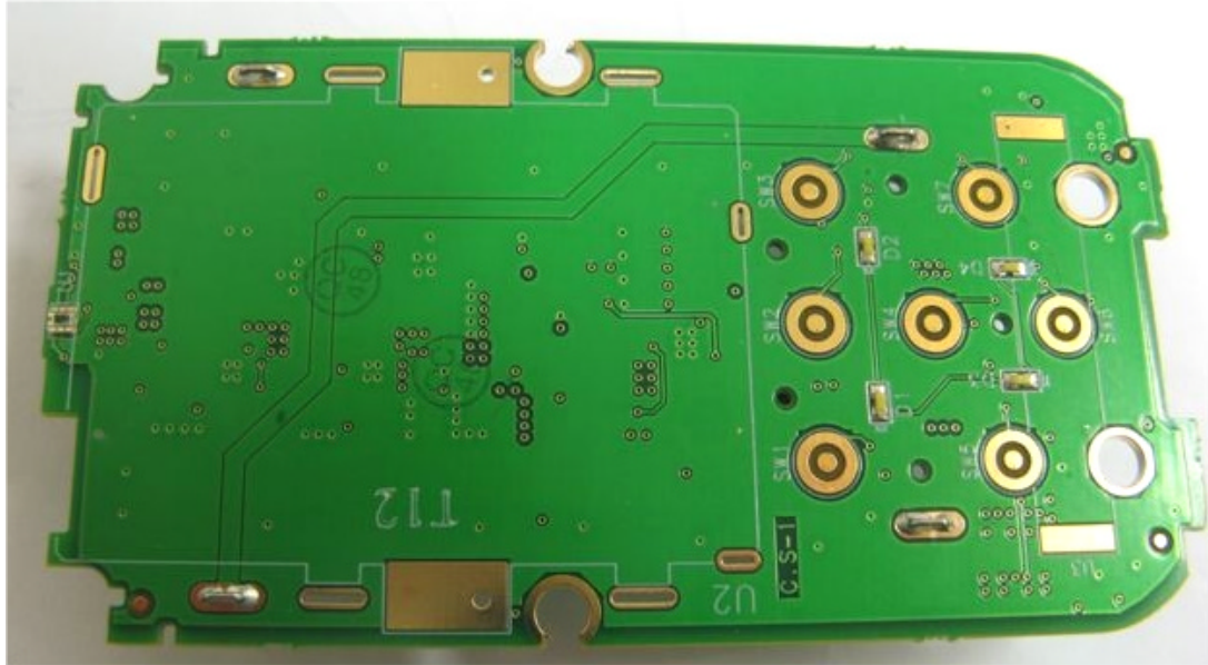
Photograph No.4 Remote Control top PCB without display view
