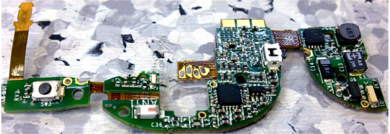
Photograph No.3 Patch pump PCB front view
