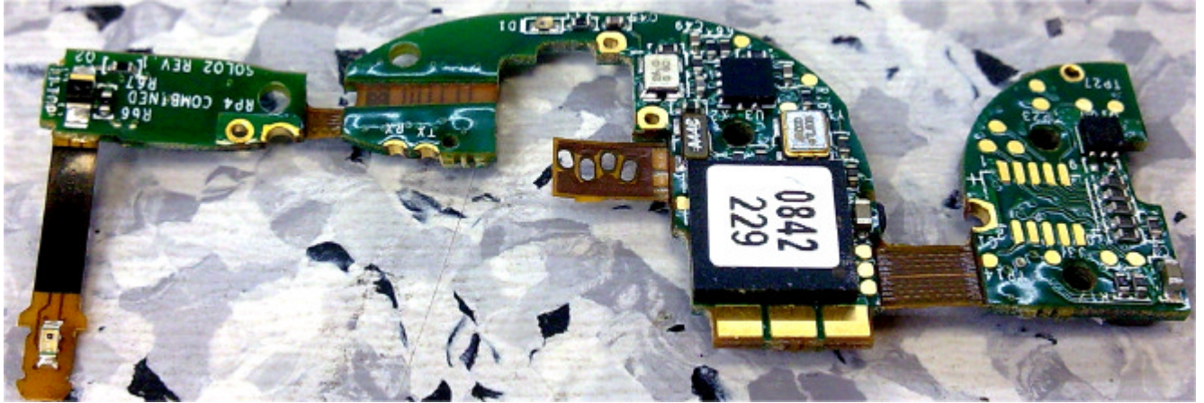
Photograph No.4 Patch pump PCB second side view
