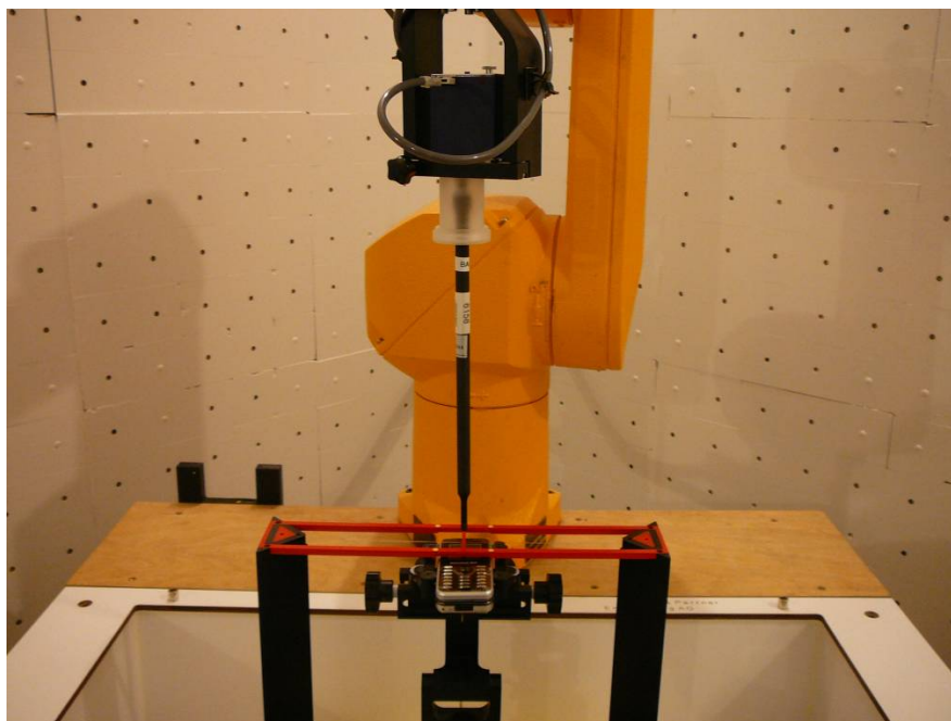
H-Field Setup View
