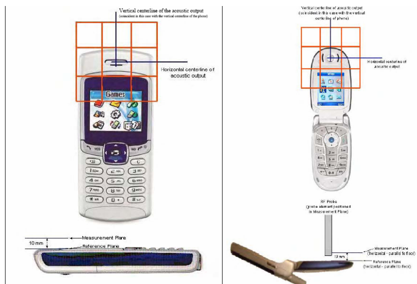
Figure 1. WD reference and plan for RF emission measurement
