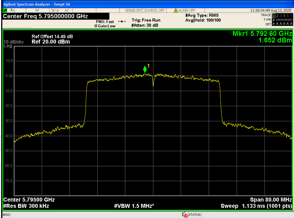
11AX40SISO-Ant1-5795-PASS
