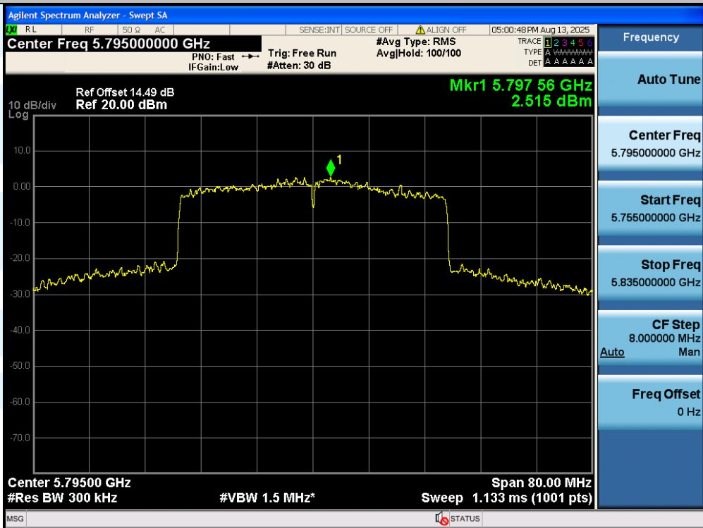
11AX40SISO-Ant2-5795-PASS
