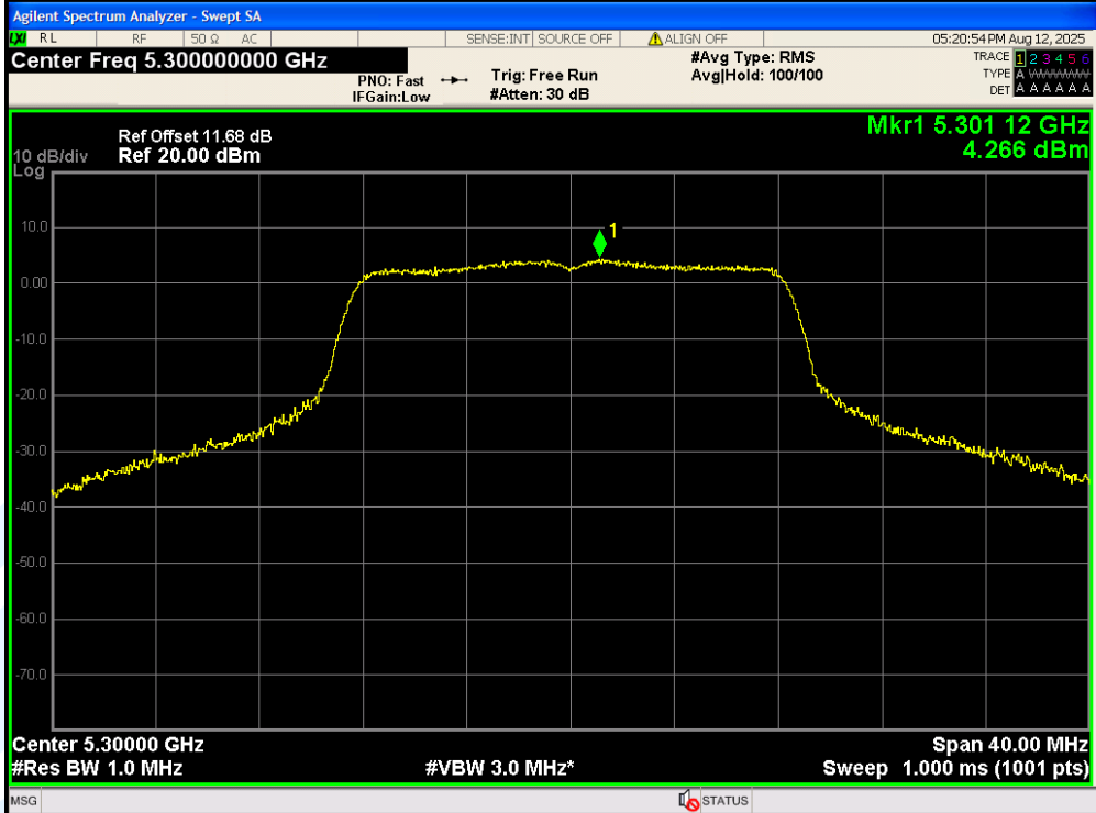
11A-Ant1-5300-PASS
