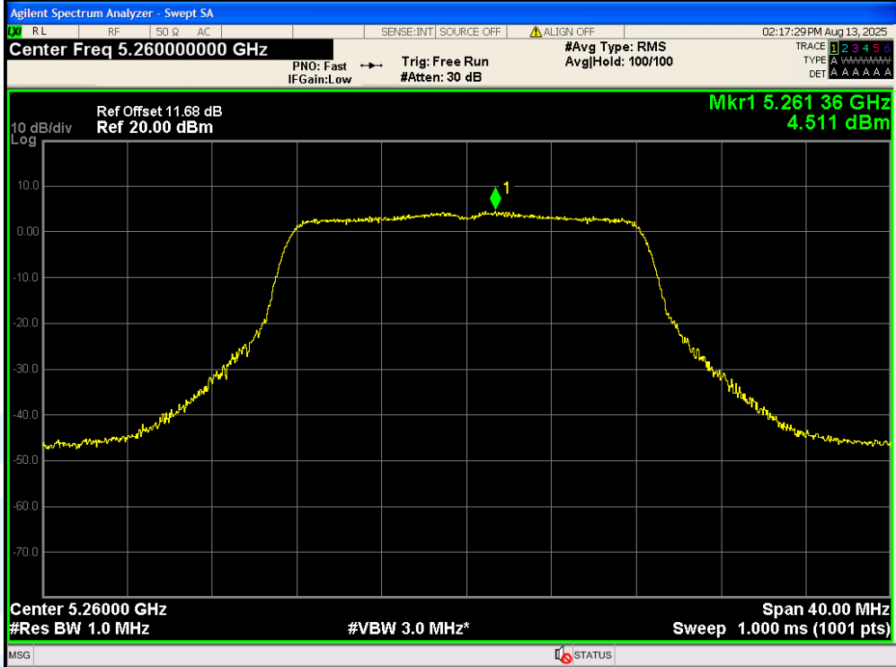
11A-Ant2-5260-PASS
