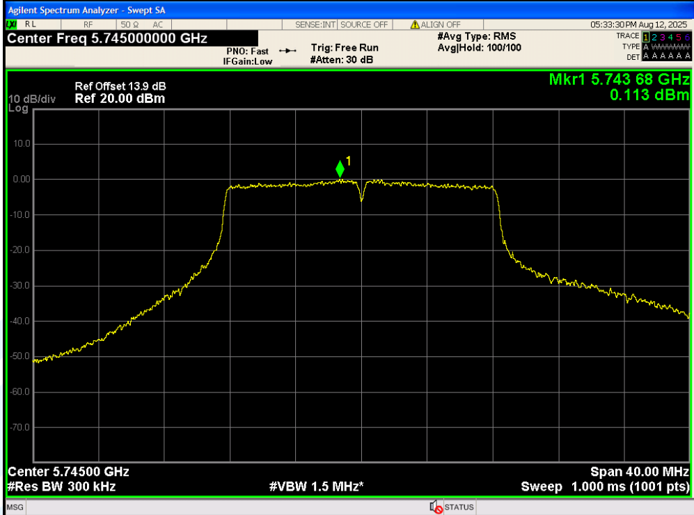
11A-Ant1-5745-PASS
