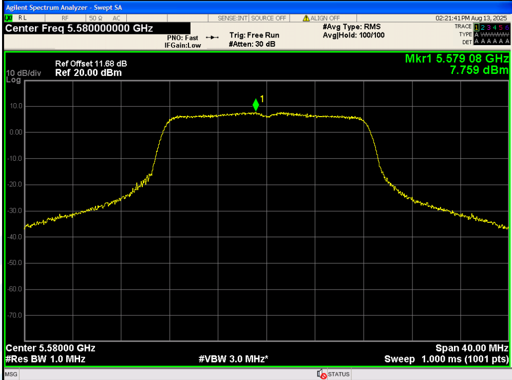
11A-Ant2-5580-PASS
