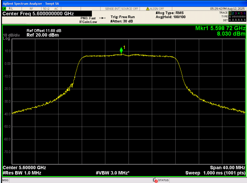
11A-Ant1-5600-PASS
