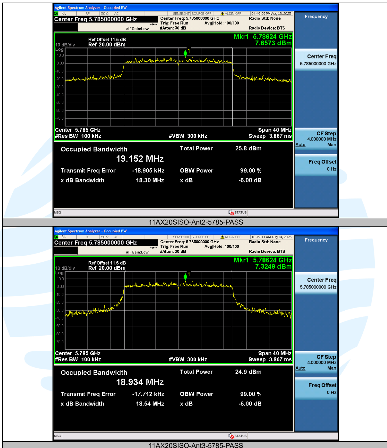
11AX20SISO-Ant3-5785-PASS
