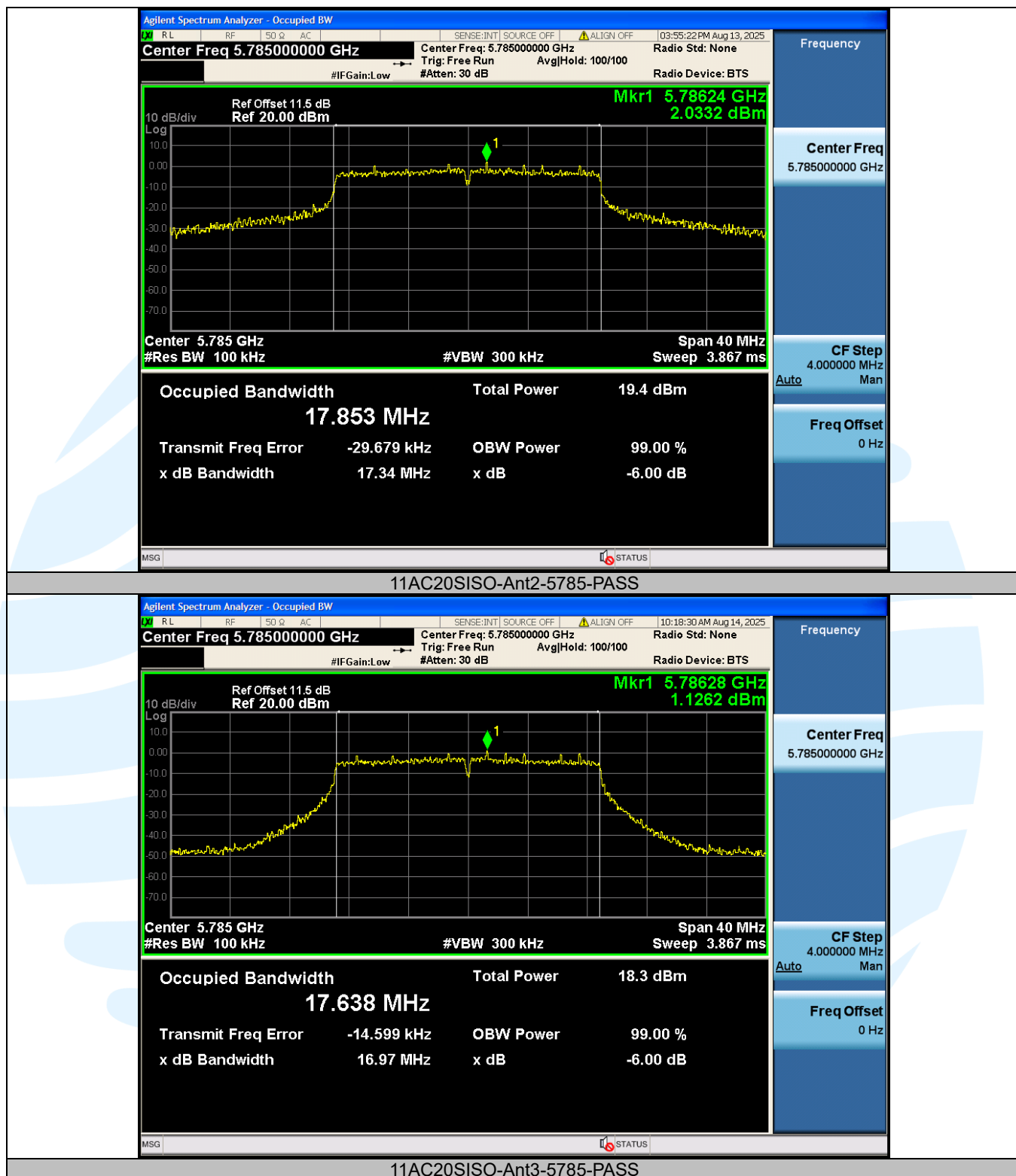
11AC20SISO-Ant3-5785-PASS
