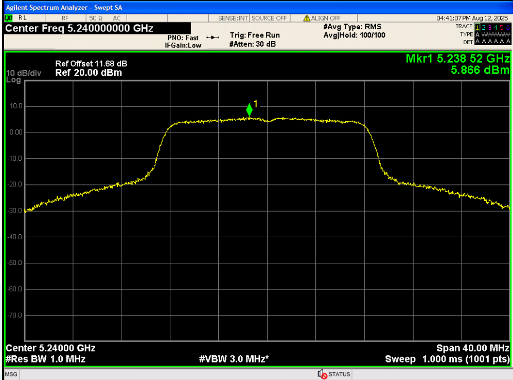
11A-Ant1-5240-PASS
