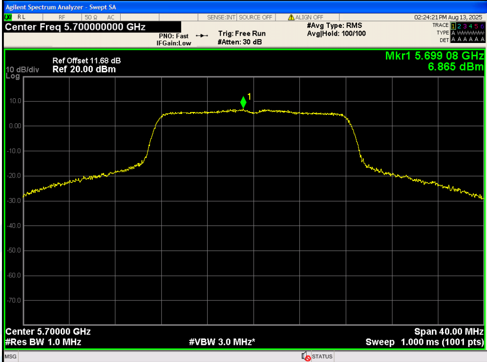
11A-Ant2-5700-PASS
