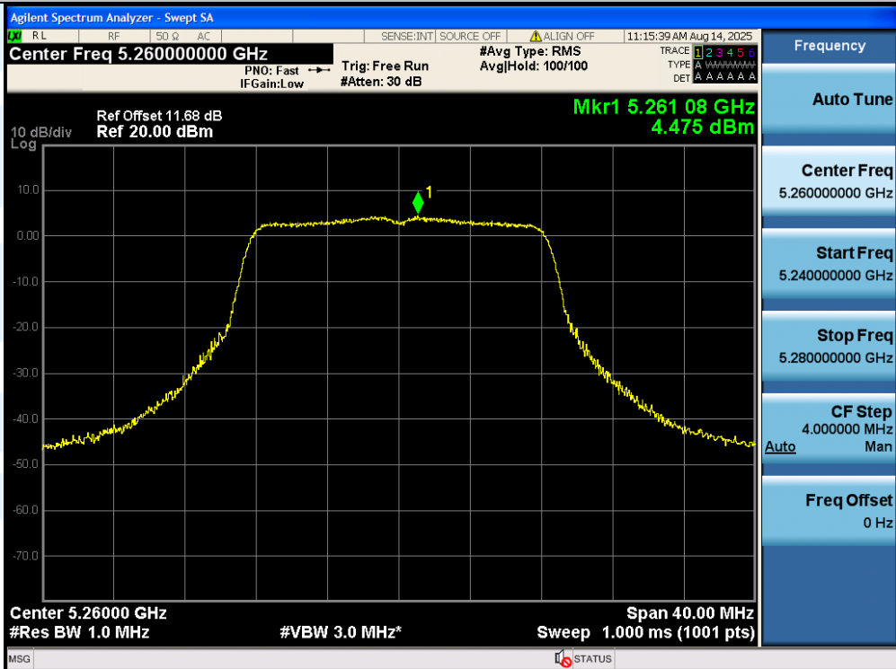
11A-Ant3-5260-PASS
