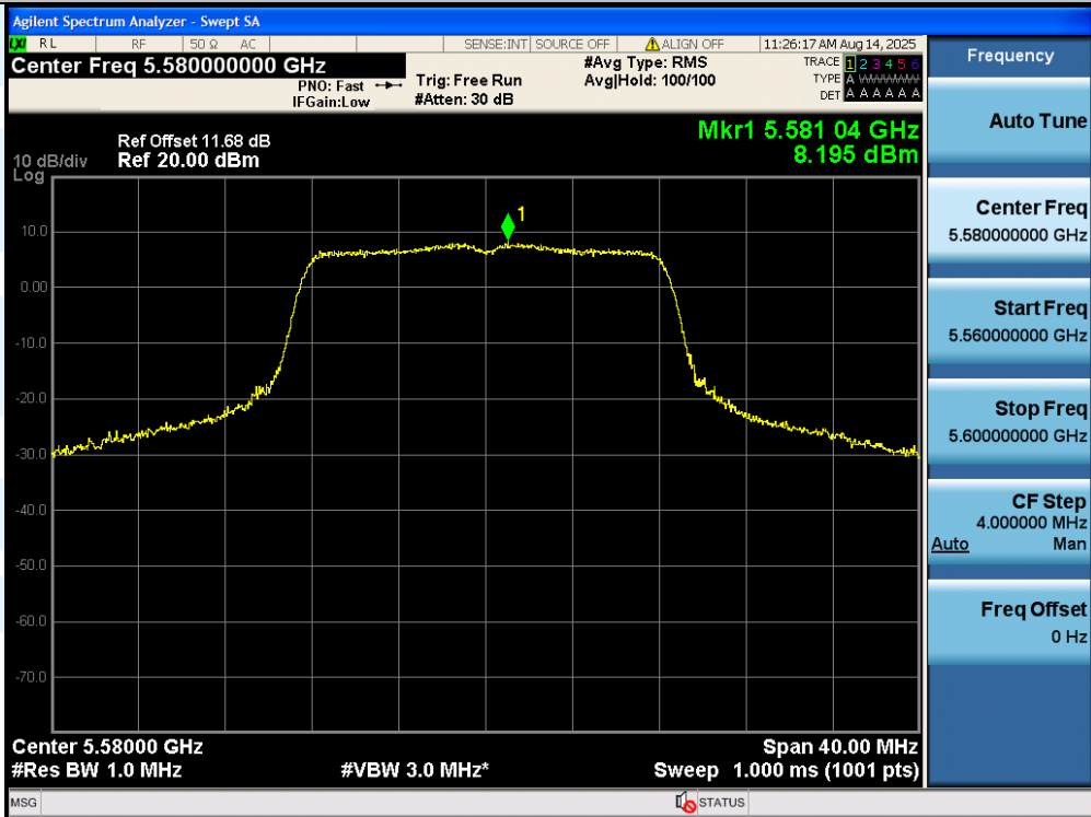
11A-Ant3-5580-PASS
