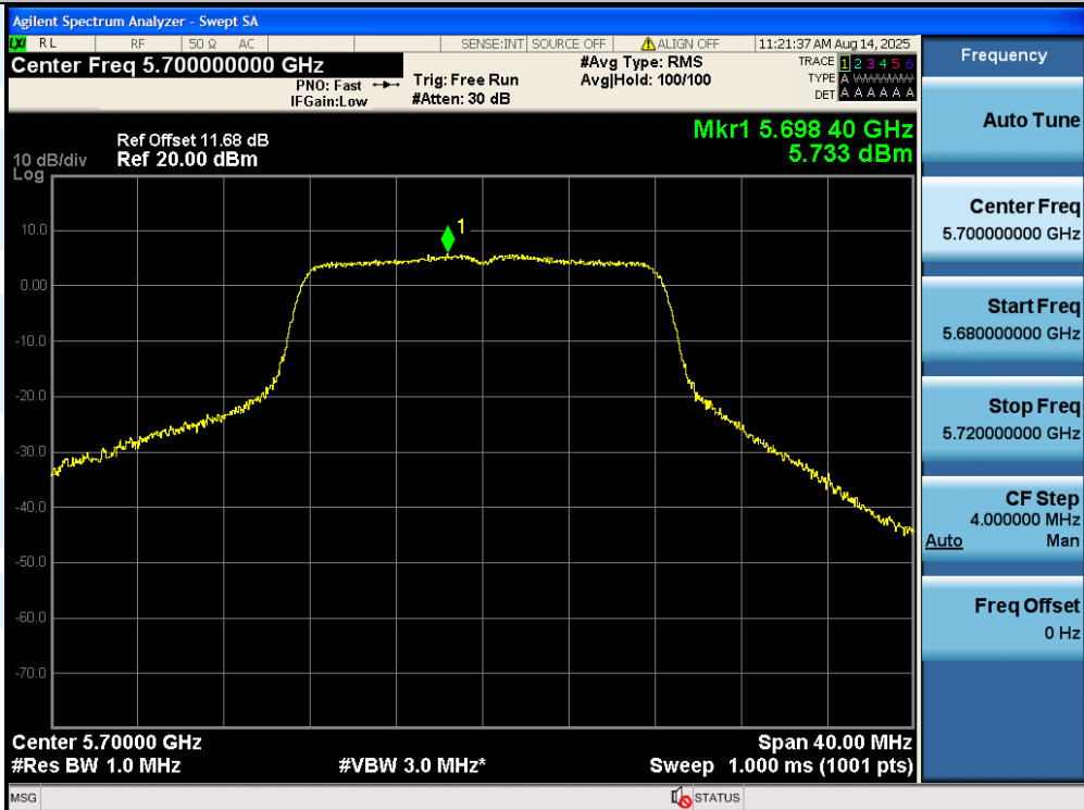
11A-Ant3-5700-PASS
