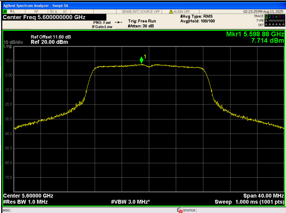
11A-Ant2-5600-PASS
