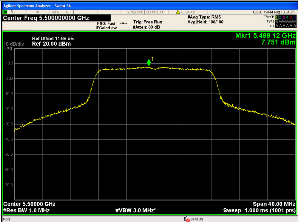
11A-Ant2-5500-PASS
