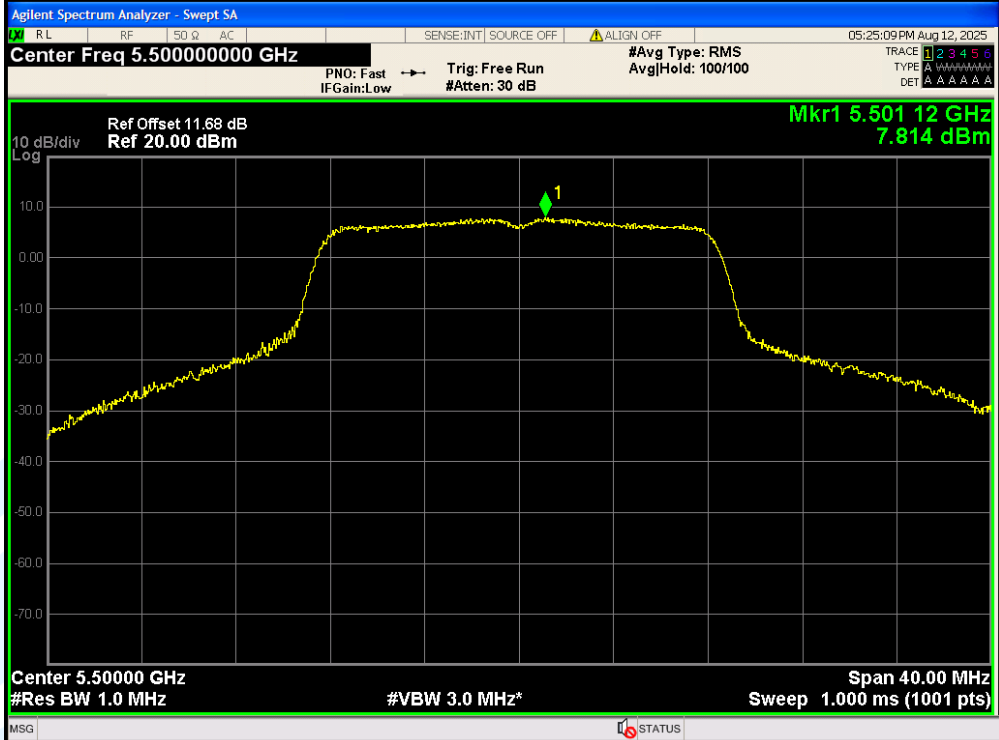
11A-Ant1-5500-PASS
