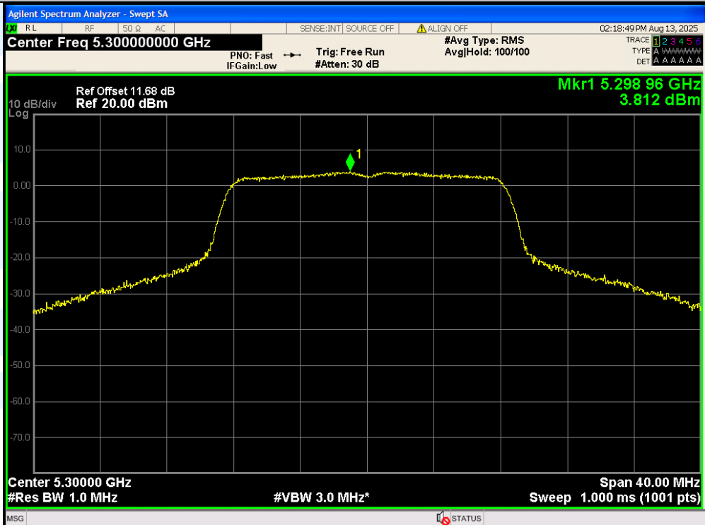
11A-Ant2-5300-PASS
