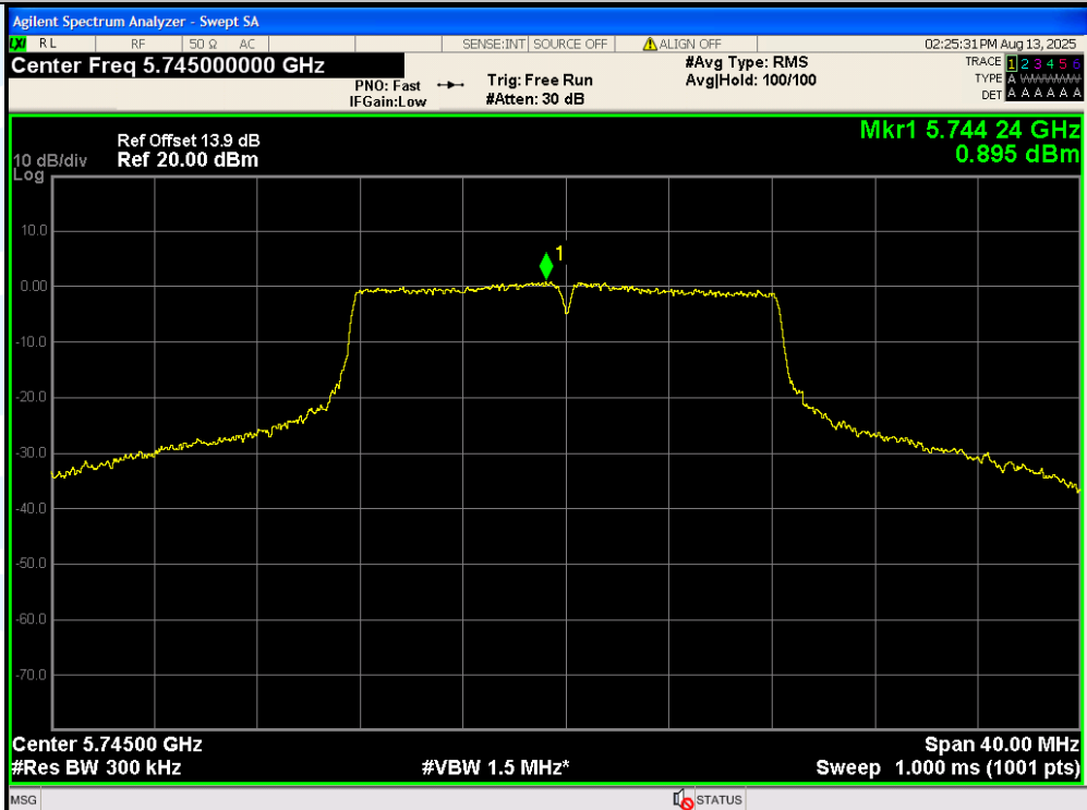
11A-Ant2-5745-PASS
