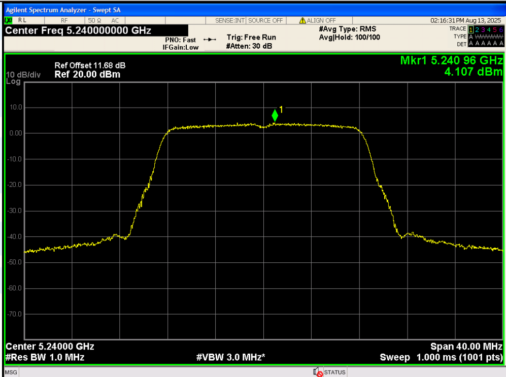
11A-Ant2-5240-PASS
