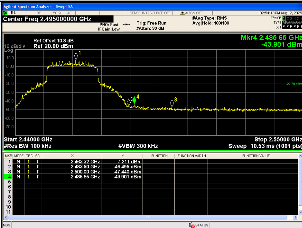
11AX20MIMO-Ant2-2462-PASS
