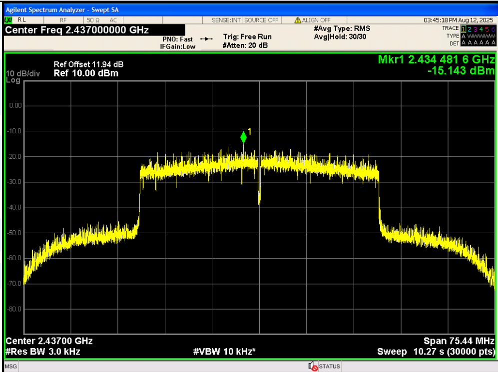
11AX40MIMO-Ant2-2437-PASS
