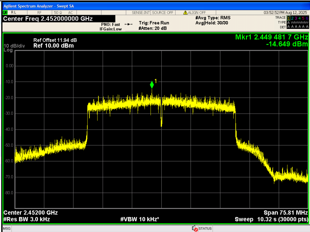
11AX40MIMO-Ant2-2452-PASS
