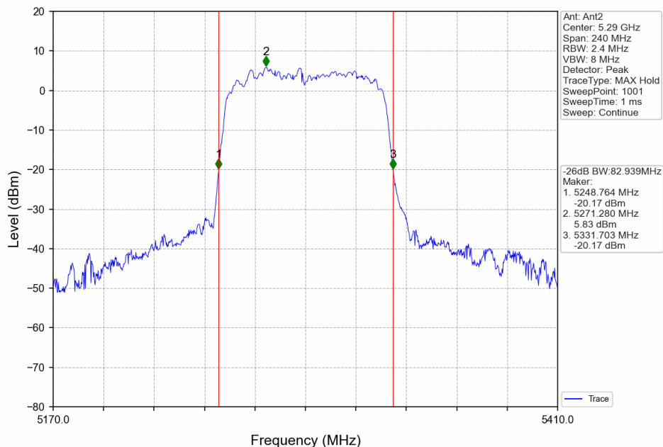
802.11ac(VHT80)_MCH_5290MHz_Ant2_NTNV
