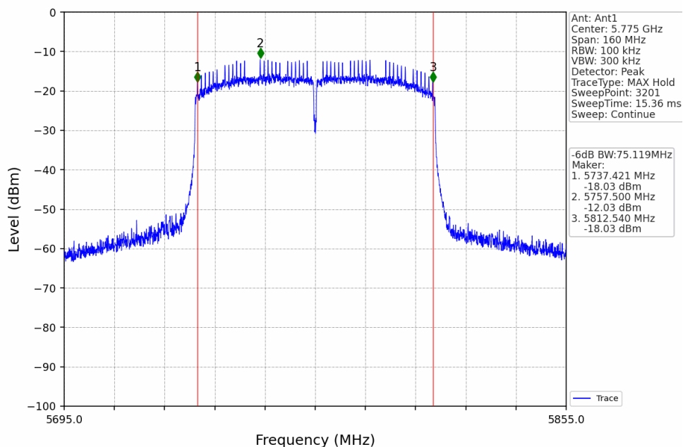
802.11ac(VHT80)_MCH_5775MHz_Ant1_NTNV
