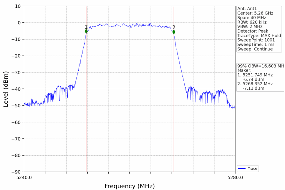
802.11a_LCH_5260MHz_Ant1_NTNV
