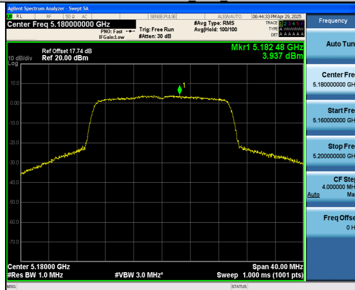
11AX20MIMO Ant2 5180
