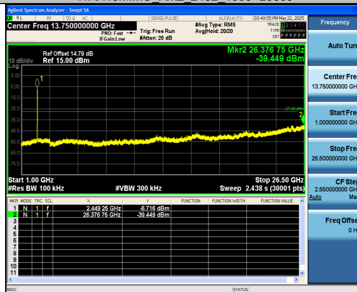
11AX40MIMO Ant2 2452 1000~26500
