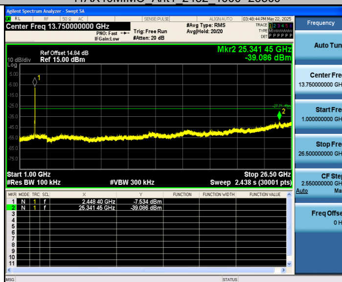
11AX40MIMO Ant2 2452 0~Reference
