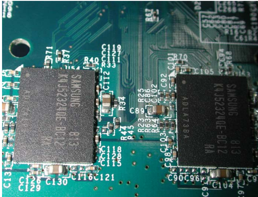
Chip View #2
