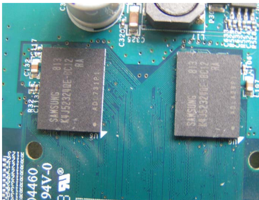
Chip View #1
