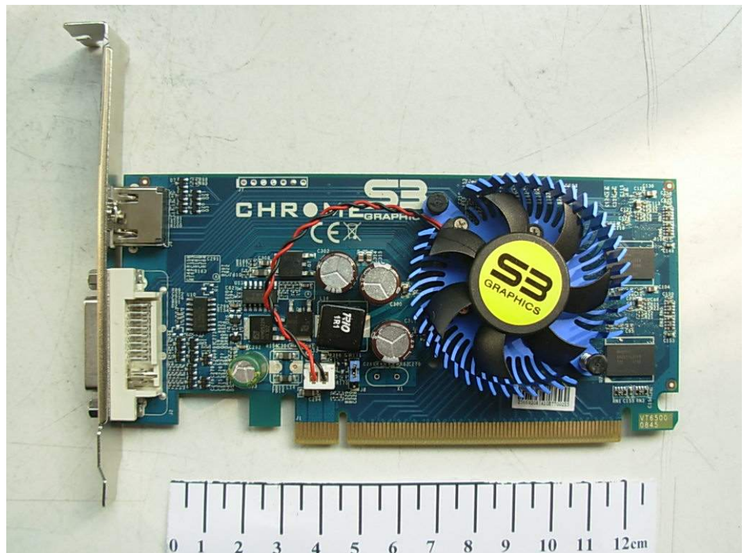
FIGURE 2 CHROME 430/440 GRAPHIC CARD (M/N: VT6500) MAIN BOARD (GENERAL APPEARANCE)
