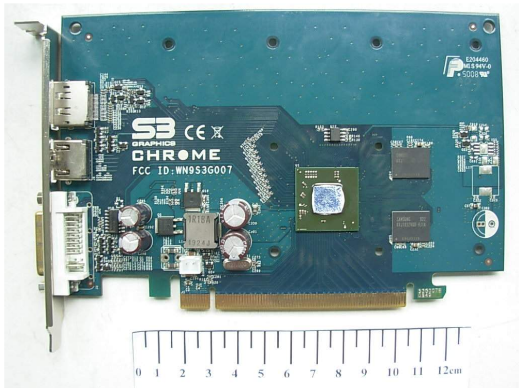
FIGURE 3 CHROME 540 GRAPHIC CARD (M/N: S3G007) MAIN BOARD (COMPONENT SIDE)
