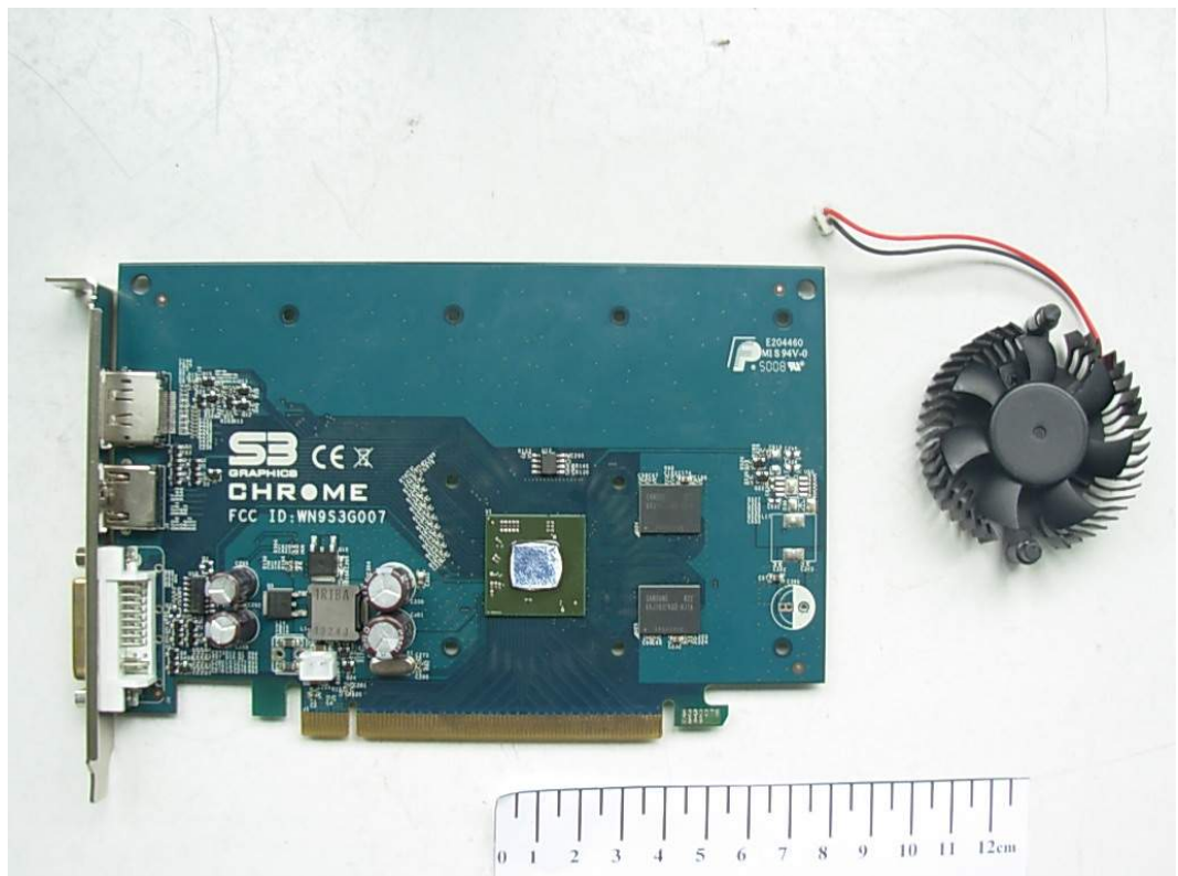
FIGURE 2 CHROME 540 GRAPHIC CARD (M/N: S3G007) MAIN BOARD CHIP FAN REMOVED
