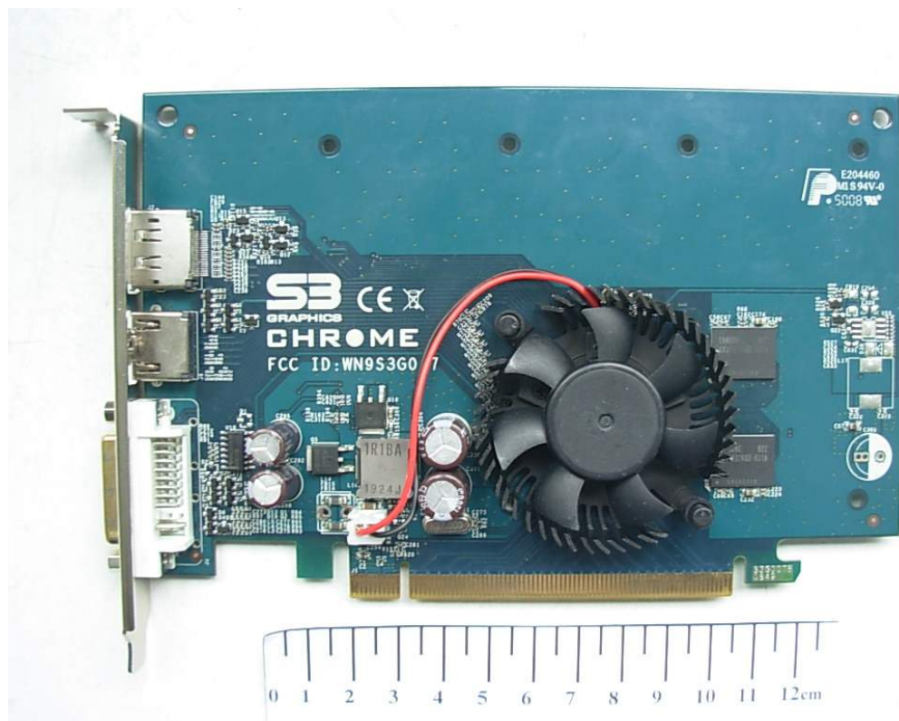
FIGURE 2 CHROME 540 GRAPHIC CARD (M/N: S3G007) MAIN BOARD (GENERAL APPEARANCE)
