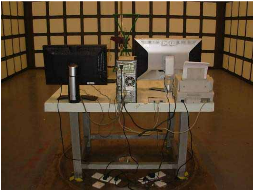
BACK VIEW OF RADIATED EMISSION TEST (BELOW 1GHZ FOR DVI+HDMI)
