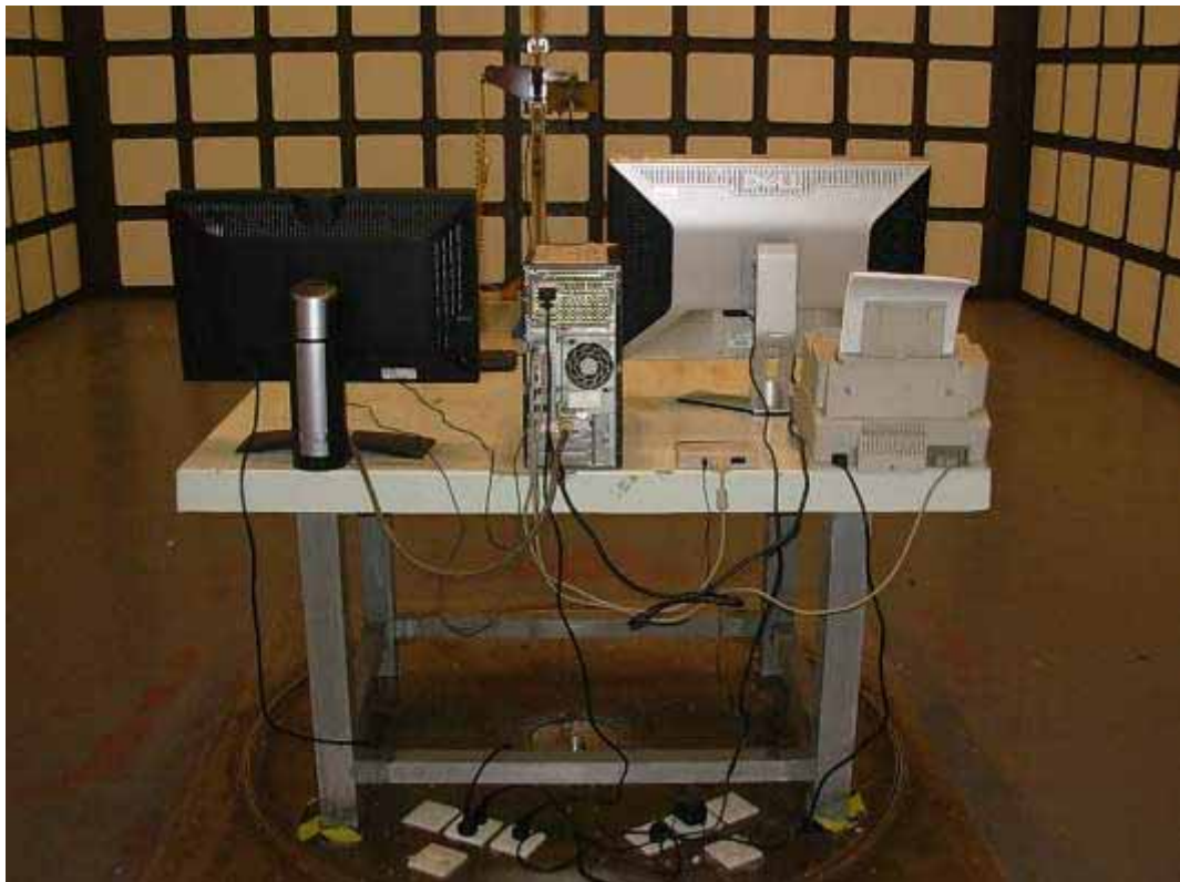
BACK VIEW OF RADIATED EMISSION TEST (ABOVE 1GHZ FOR DVI+HDMI)
