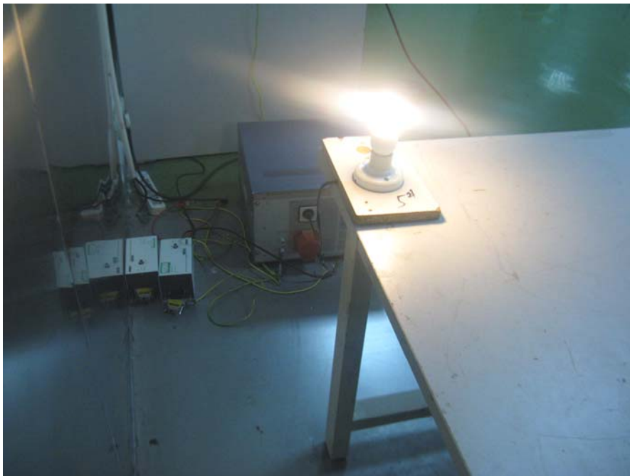
ELT-N809: Conducted Emissions - Side View
