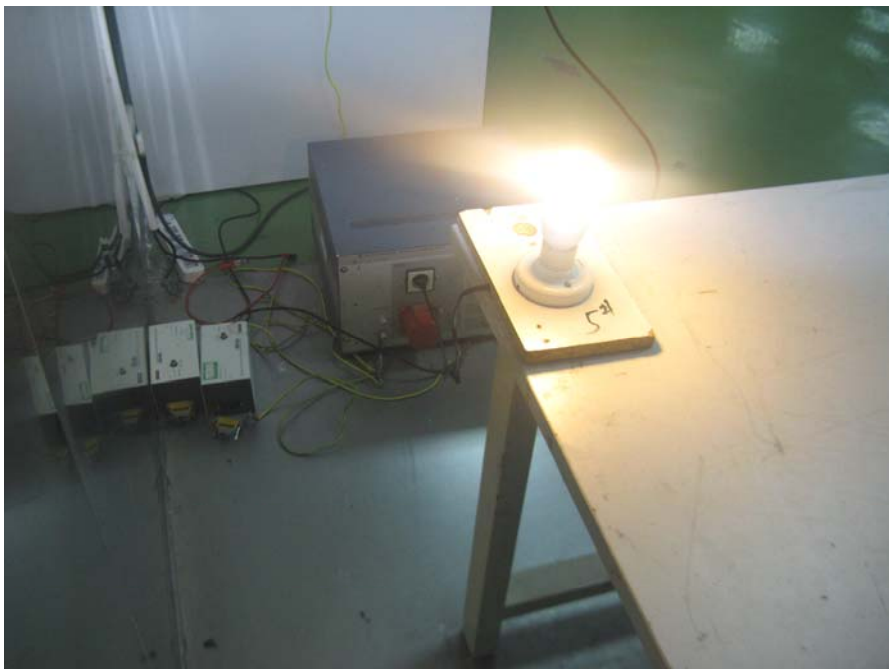
ELT-N811: Conducted Emissions - Side View
