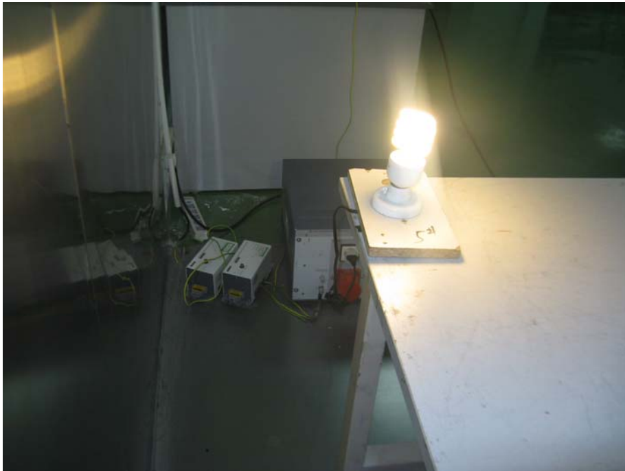
ELT-N920: Conducted Emissions - Side View
