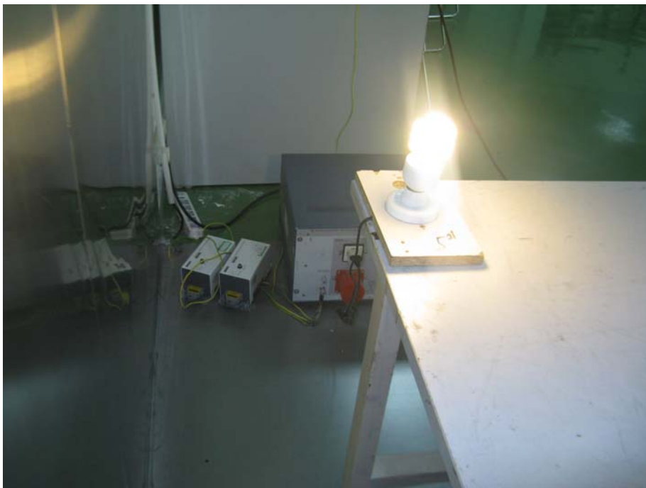
ELT-N923: Conducted Emissions - Side View
