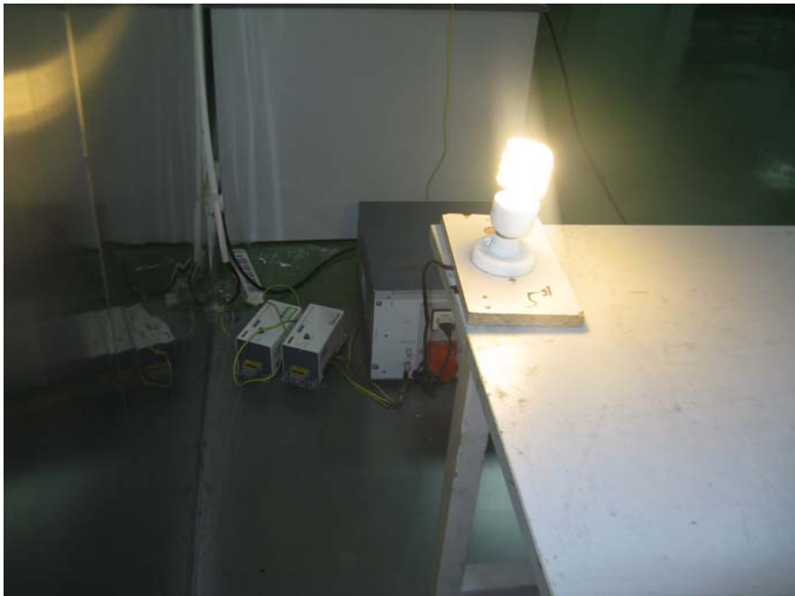
ELT-N820: Conducted Emissions - Side View
