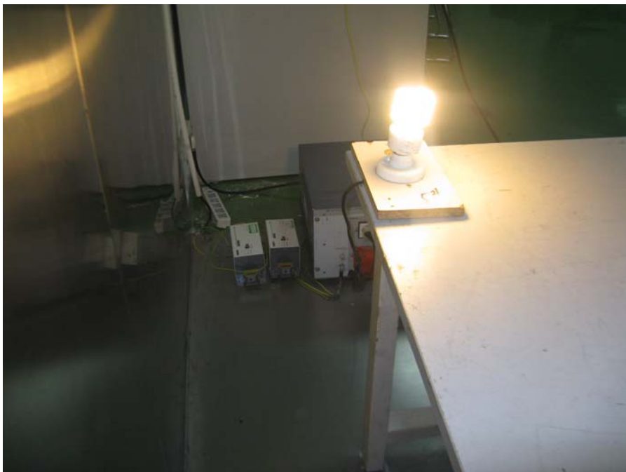
ELT-N818: Conducted Emissions - Side View
