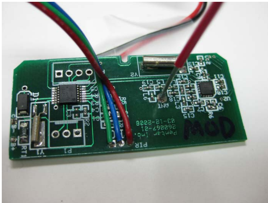
Close-Up of RF Section View #2
