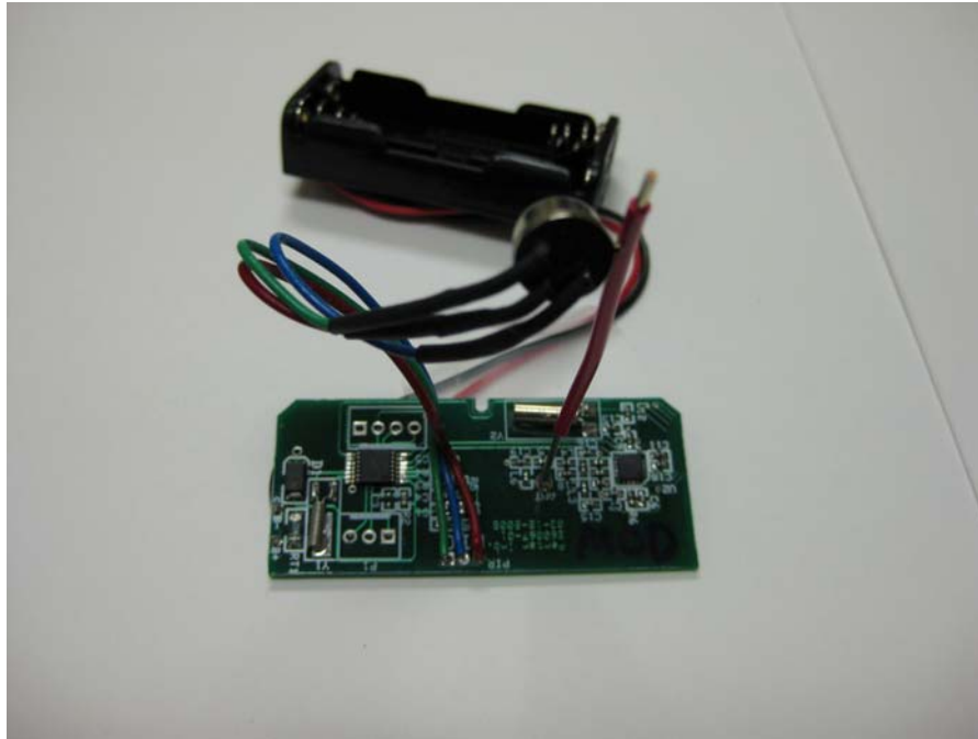
RF Section View #1
