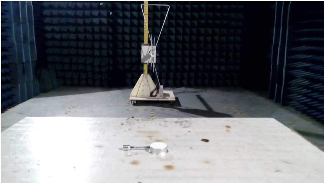
Radiated Emissions (Below 1GHz)
