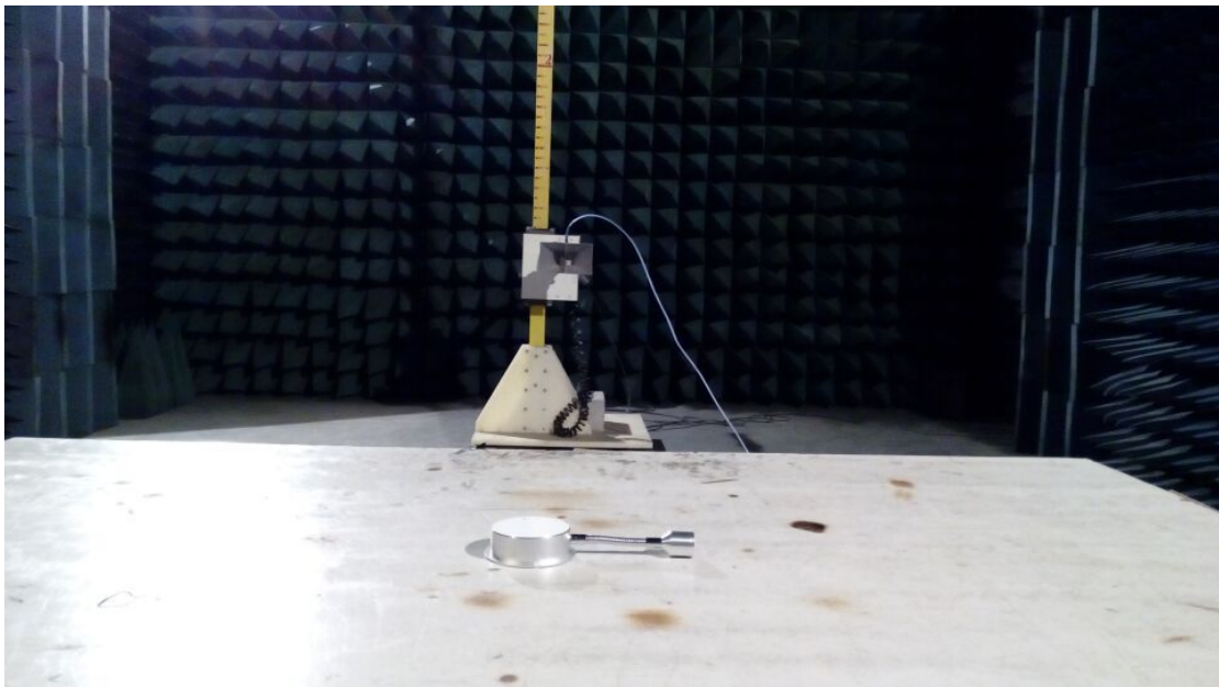
Radiated Emissions (Above 1GHz)
