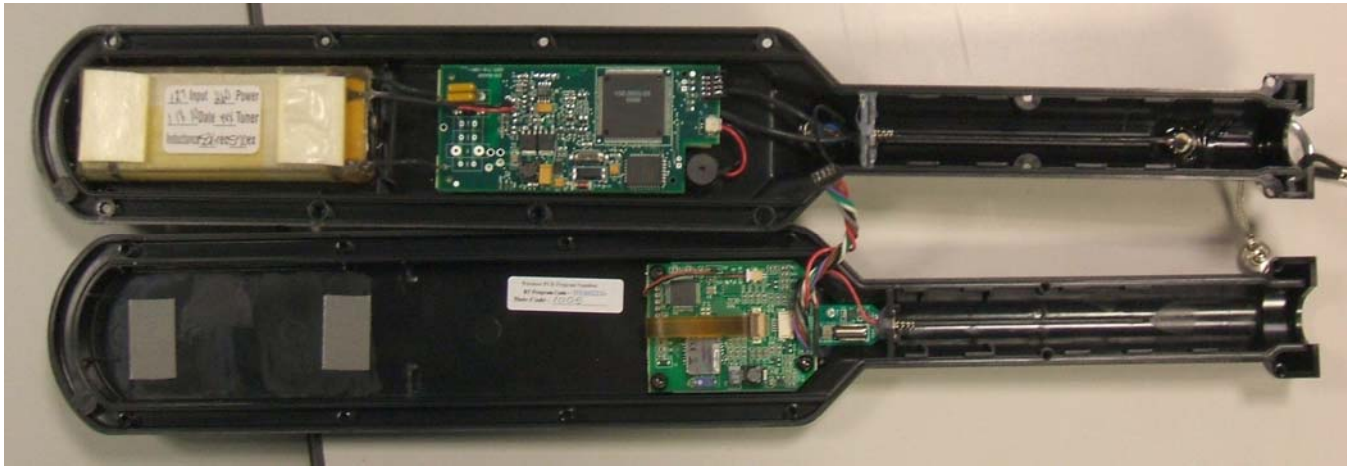
READER BOARD FRONT
