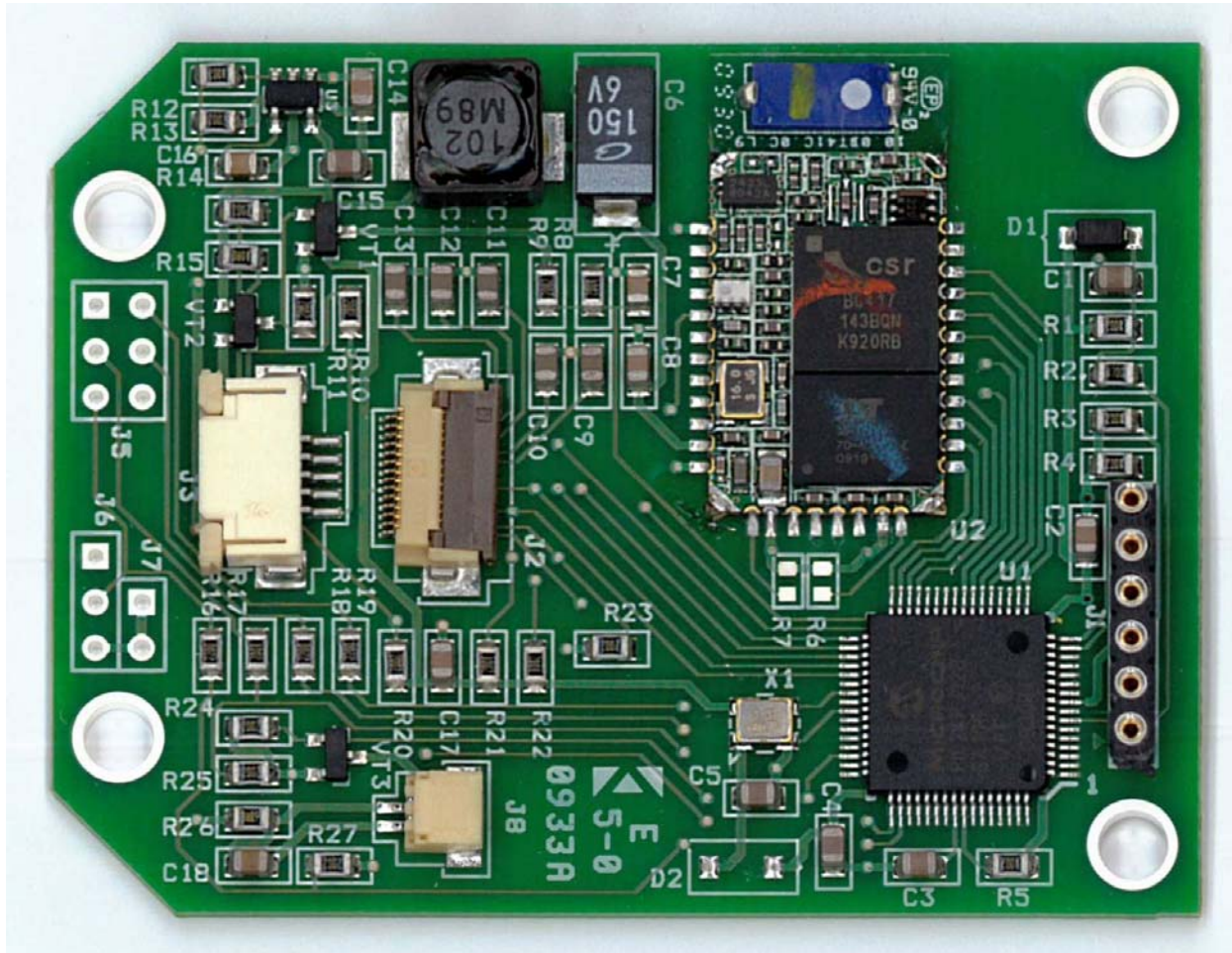
Display board with Bluetooth shield off
