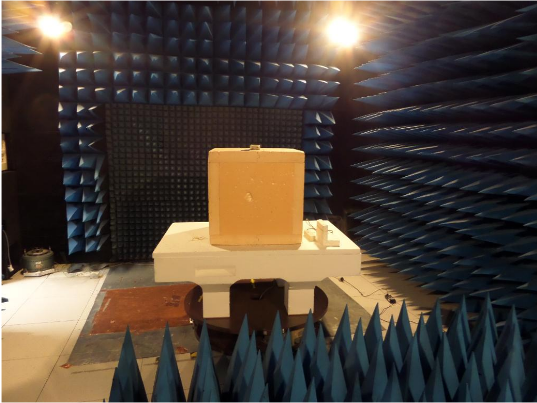
Anechoic chamber - TX mode
