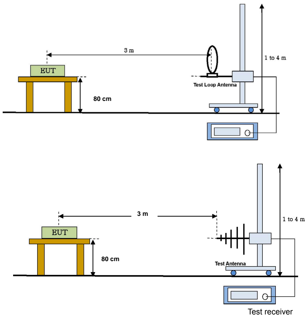
[ Radiated emission setup ]
