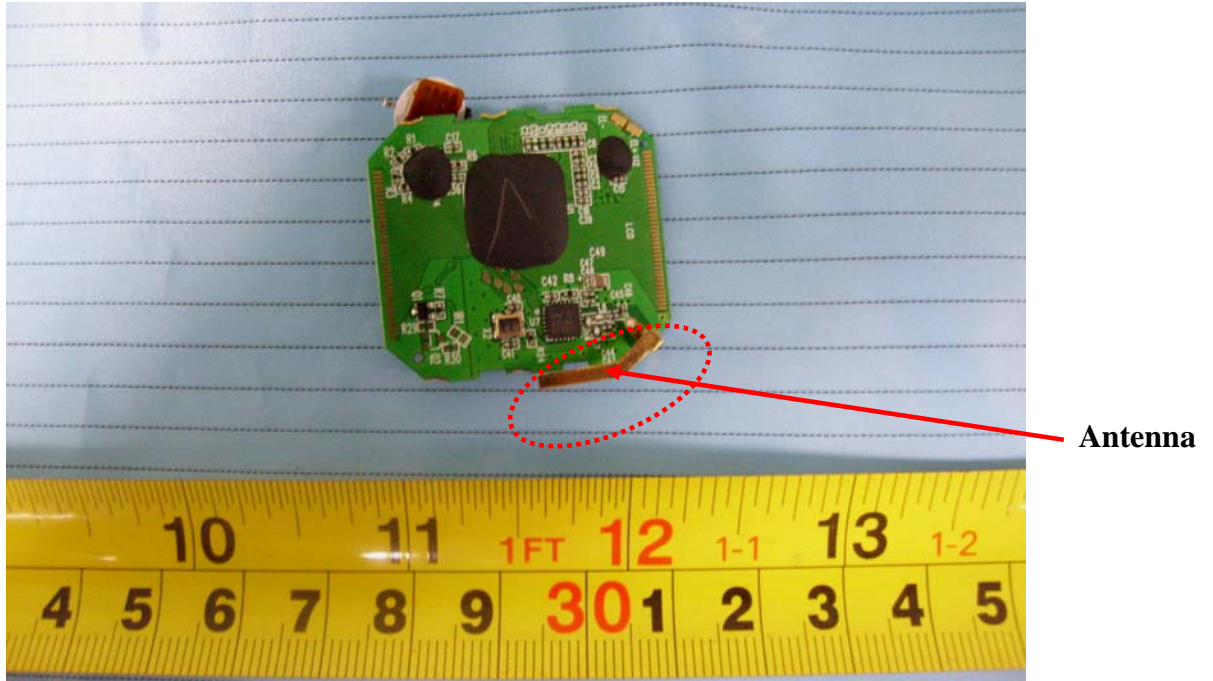
EUT – Main Board Top Components View
