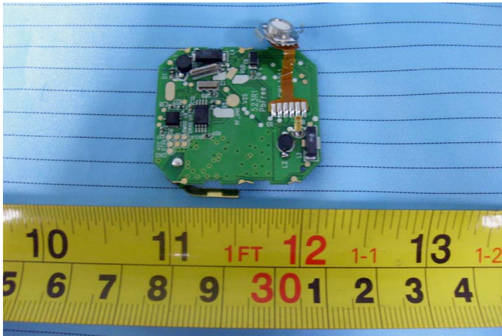
EUT – Main Board Bottom Components View
