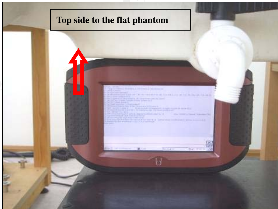
Fig.3 Configuration 1: Top side of EUT is paralleled with flat phantom, top side is contact with flat phantom.
