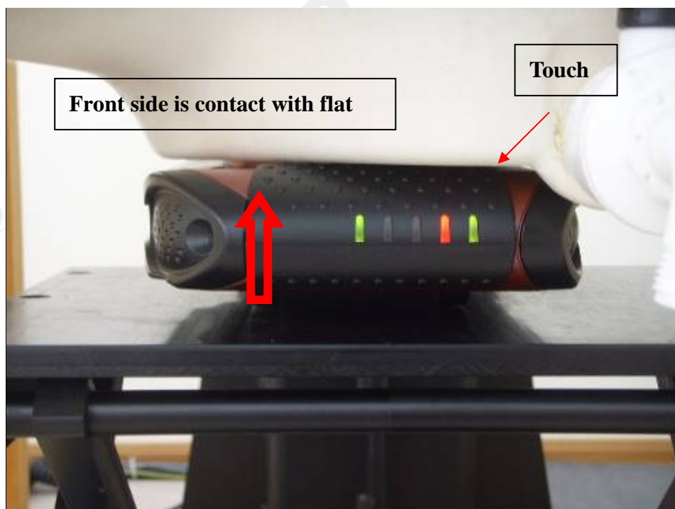
Fig.5 Configuration 2: Front side of EUT is paralleled with flat phantom, Front side is contact with flat phantom.
