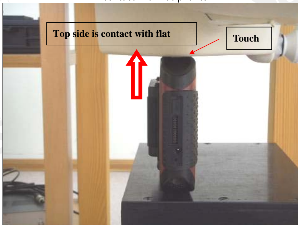
Fig.4 Configuration 1: Top side of EUT is paralleled with flat phantom, top side is contact with flat phantom.
