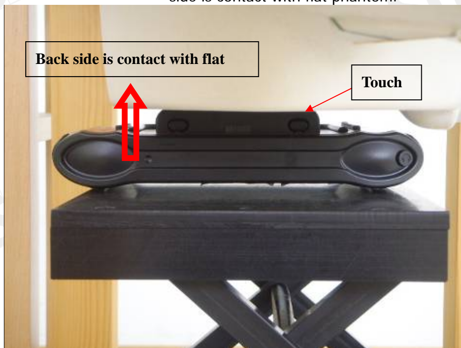
Fig.8 Configuration 3: Back side of EUT is paralleled with flat phantom , Back side is contact with flat phantom.
